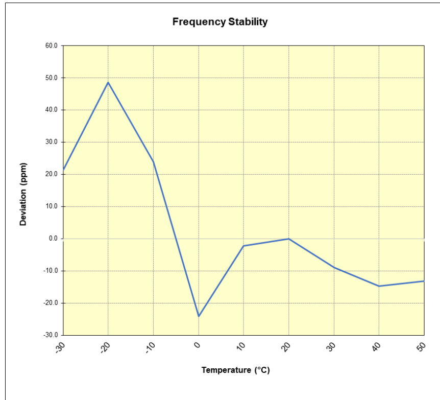
Plot 7-27. LTE Band 41(PC3) Frequency Stability Chart
