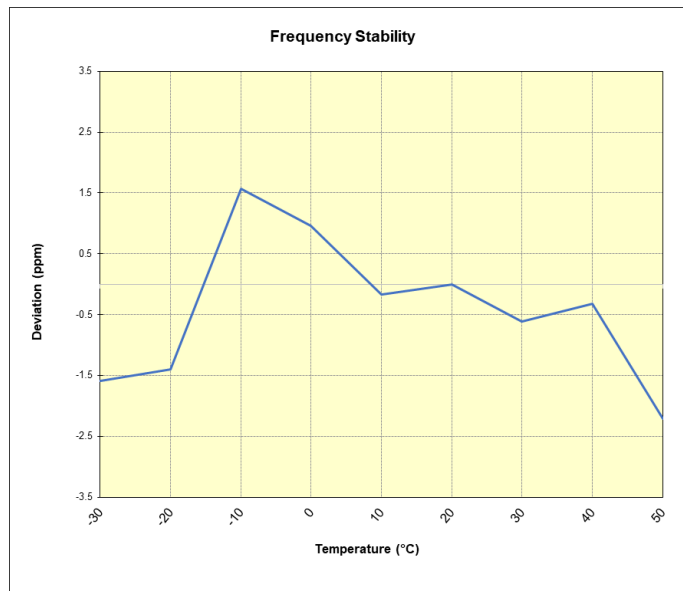
Plot 7-60. WCDMA Cell Frequency Stability Chart
