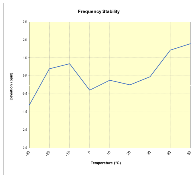
Plot 7-59. GSM/GPRS Cell Frequency Stability Chart
