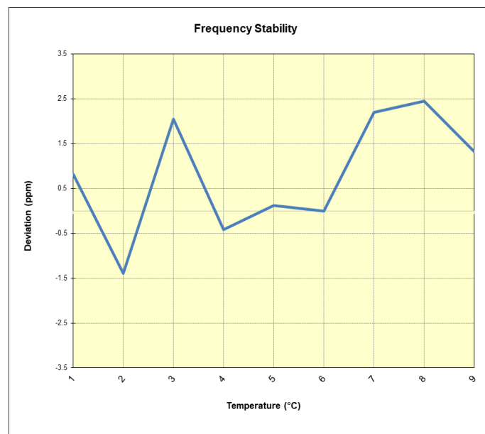
Plot 7-58. LTE Band 26/5 Frequency Stability Chart
