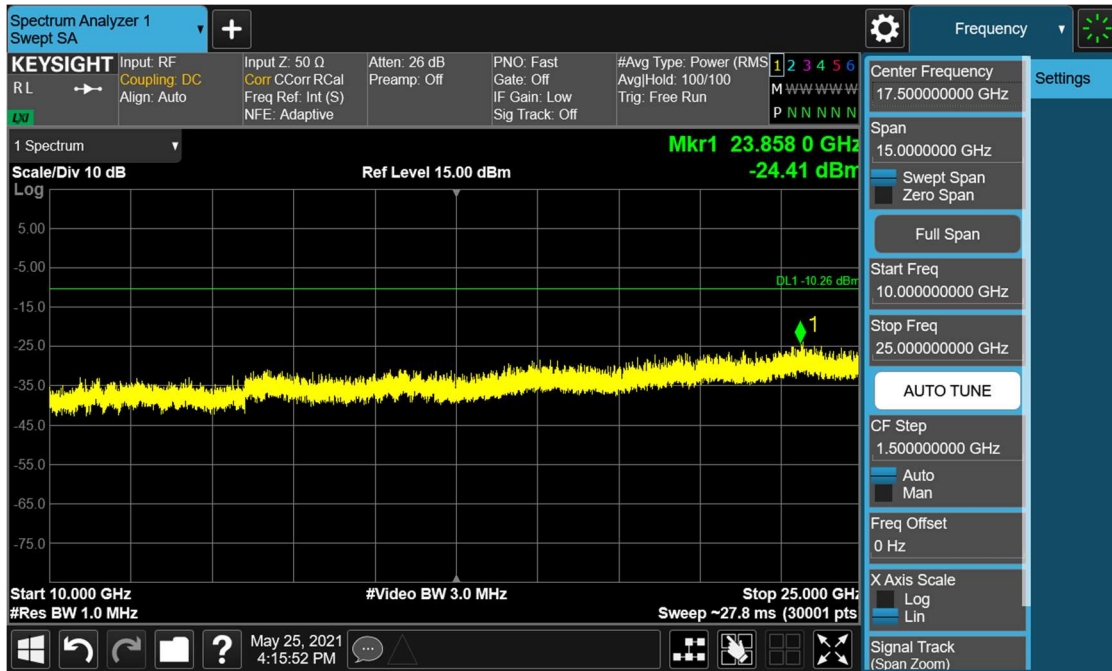
Plot 7-39. Conducted Spurious Plot (Bluetooth, 3Mbps – Ch. 39)
