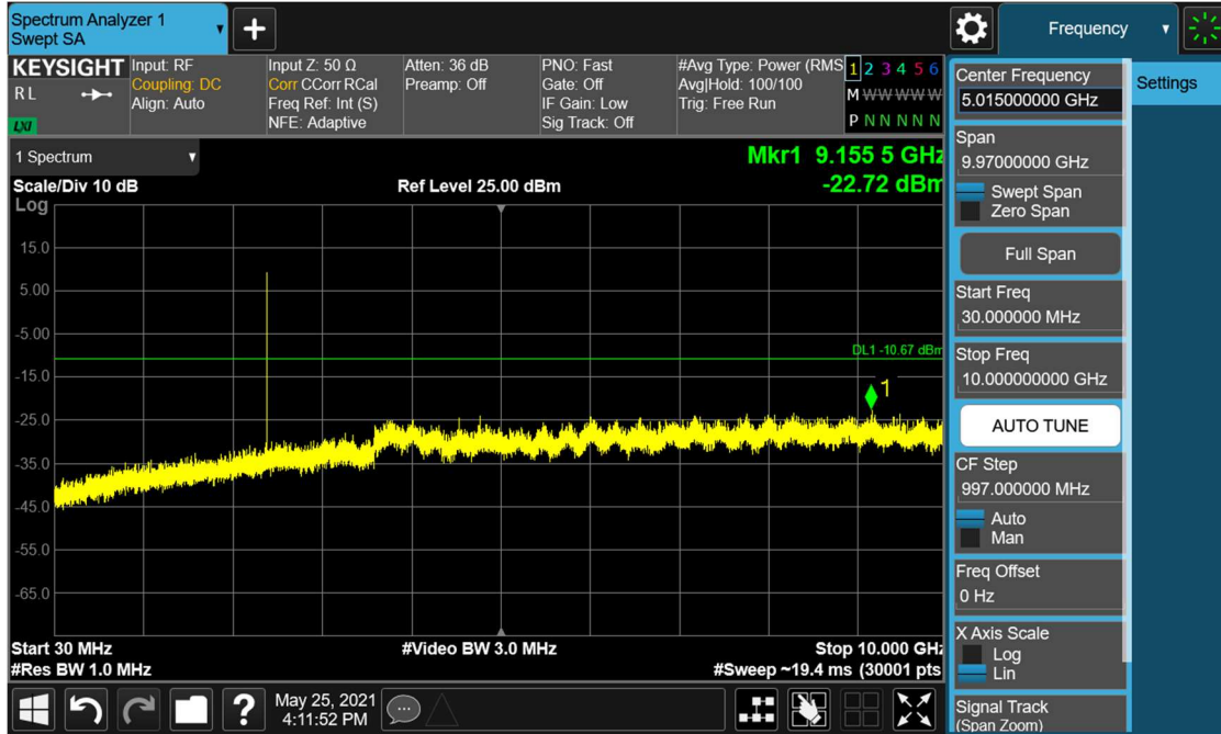
Plot 7-36. Conducted Spurious Plot (Bluetooth, 3Mbps – Ch. 0)
