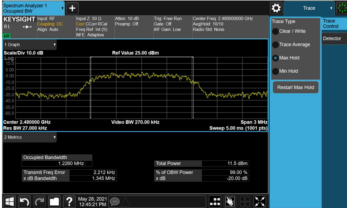
Plot 7-6. 20dB Bandwidth Plot (Bluetooth, 2Mbps – Ch. 78)
