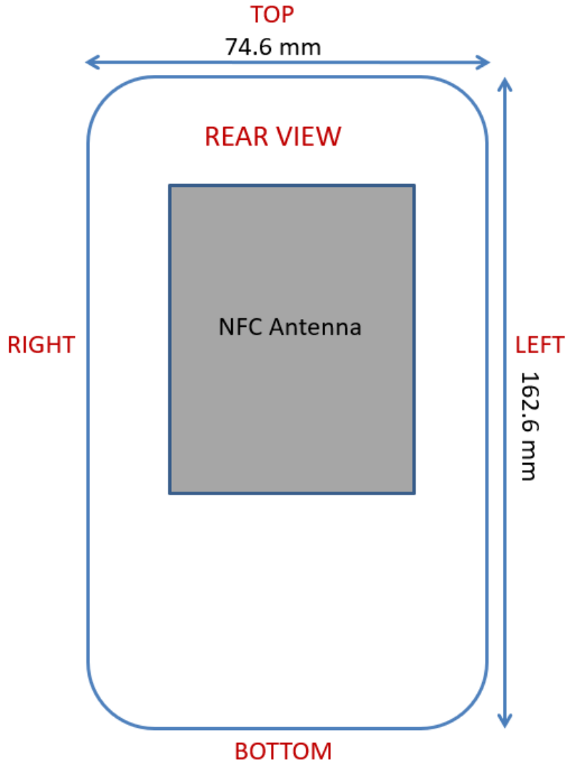
Figure E-2 NFC Antenna Locations
