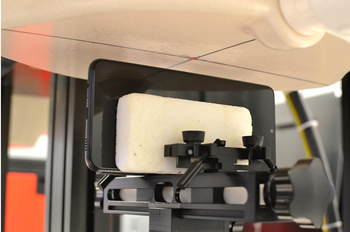
SAR Test Setup Photo 15 – Phablet, Left Edge at 11 mm
