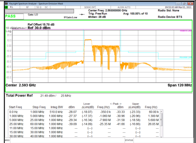
LTE B41 5MHz + 20MHz QPSK Mid Ch RB25-0 + RB100-0
