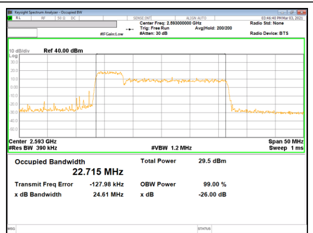
LTE B41 5MHz + 20MHz 16QAM RB25-0 + RB100-0
