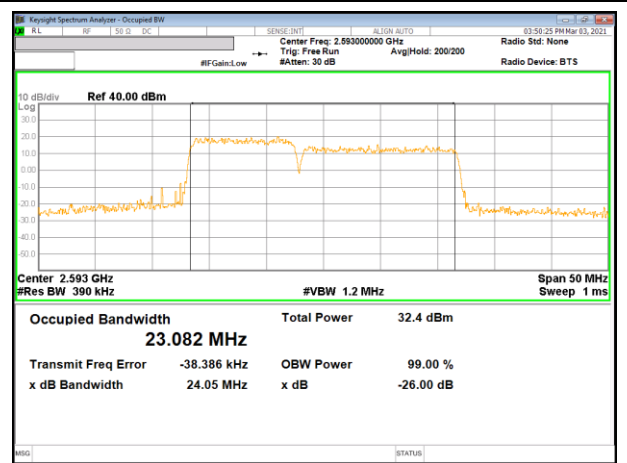
LTE B41 10MHz + 15MHz 16QMA RB50-0 + RB75-0
