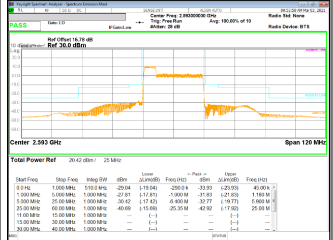
LTE B41 5MHz + 20MHz 16QAM Mid Ch RB25-0 + RB100-0
