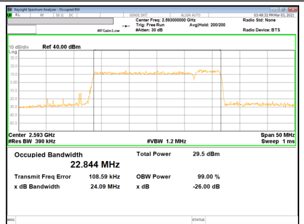
LTE B41 20MHz + 5MHz 16QAM RB100-0 + RB25-0
