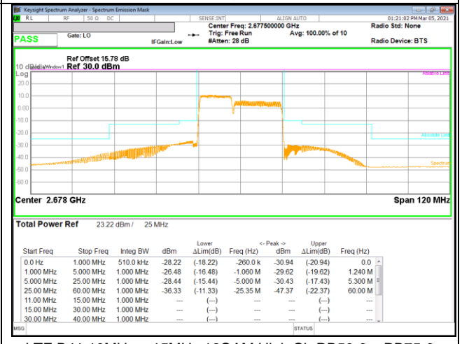
LTE B41 10MHz + 15MHz 16QAM High Ch RB50-0 + RB75-0
