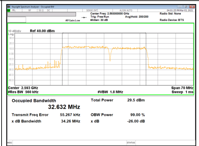
LTE B41 20MHz + 15MHz 16QAM RB100-0 + RB75-0
