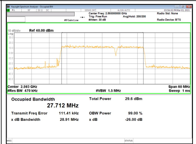
LTE B41 20MHz + 10MHz 16QAM RB100-0 + RB50-0
