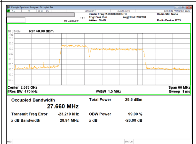
LTE B41 10MHz + 20MHz 16QAM RB50-0 + RB100-0
