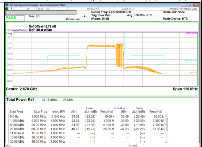
LTE B41 20MHz + 5MHz QPSK High Ch RB100-0 + RB25-0
