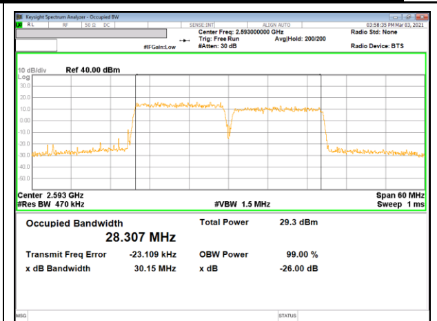
LTE B41 15MHz + 15MHz 16QAM RB75-0 + RB75-0
