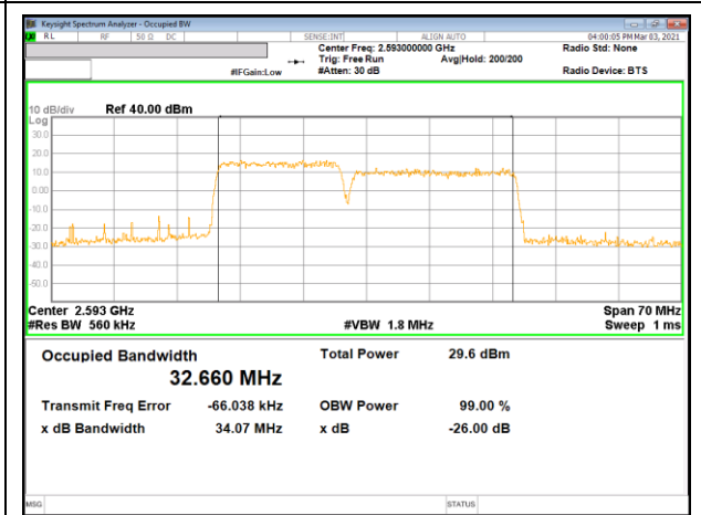
LTE B41 15MHz + 20MHz 16QAM RB75-0 + RB100-0
