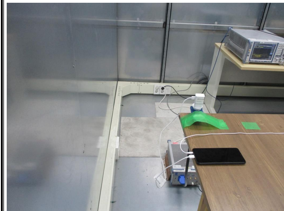
AC LINE CONDUCTED REAR TEST PHOTO
