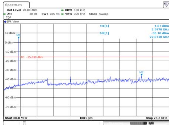
Conducted spurious / Mid ch.
