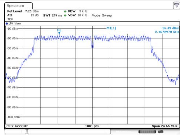
802.11g / 2 472 MHz
