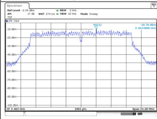
802.11g / 2 462 MHz
