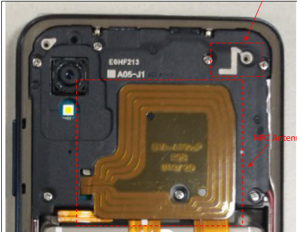
WLAN/BT/BLE Antenna (LDS)
