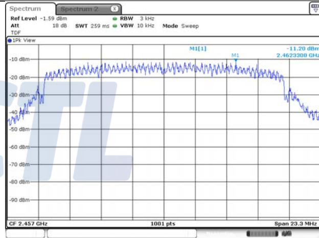
802.11n HT20 / 2 457 MHz
