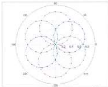
f=600 MHz,TEM
