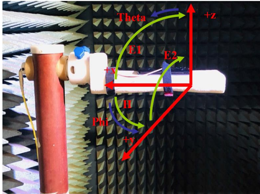
Figure 4: Geometry for SM-A047F for Radiation patterns.
