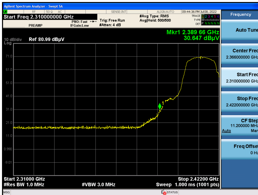
Radiated Restricted Band Edges plot – Peak Result (802.11g_6 Mbps Ch.1, X-H)
