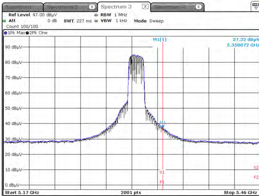
Average Result (802.11a, Ch.64 Spurious Emissions, X-H)
