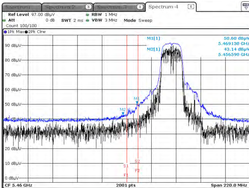
Peak Result (802.11ac(VHT20), Ch.100 Spurious Emissions, Y-H)
