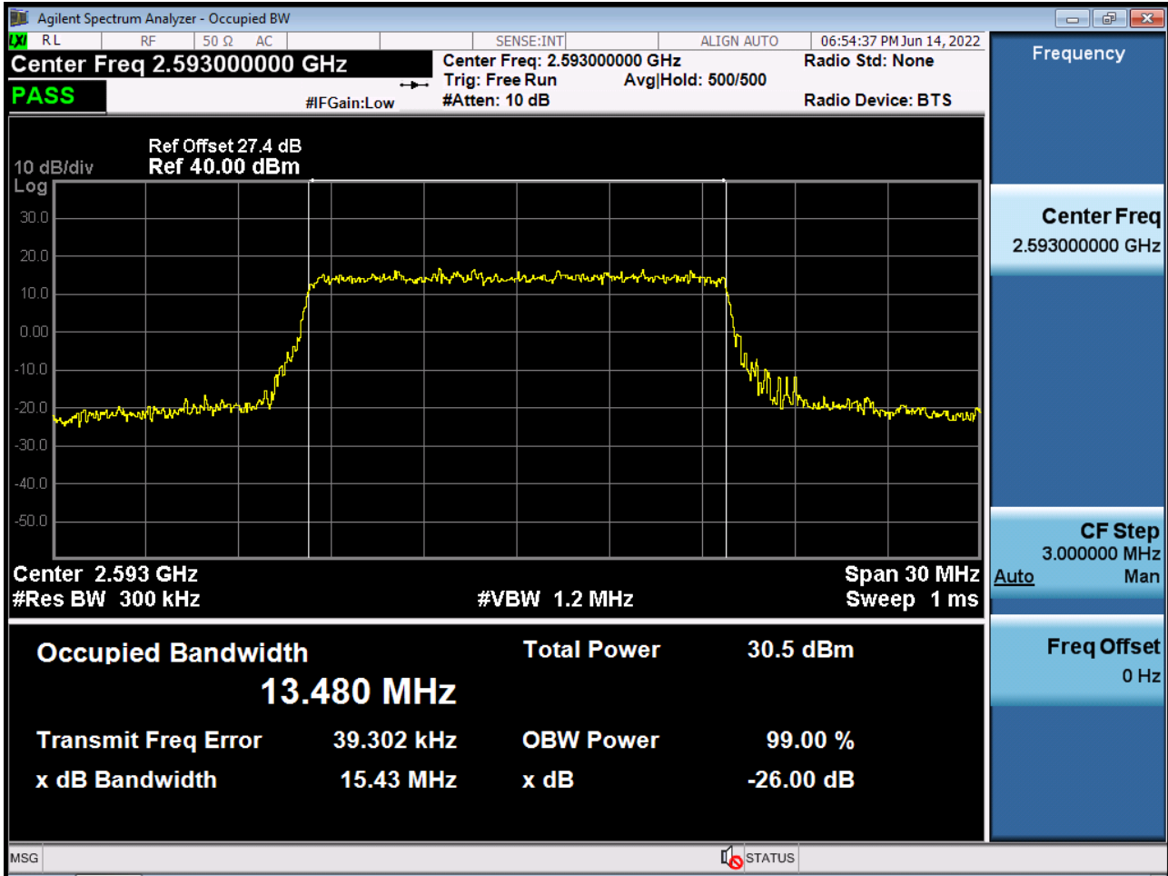
Occupied Bandwidth Plot (15 MHz Ch.40620 QPSK RB 75)
