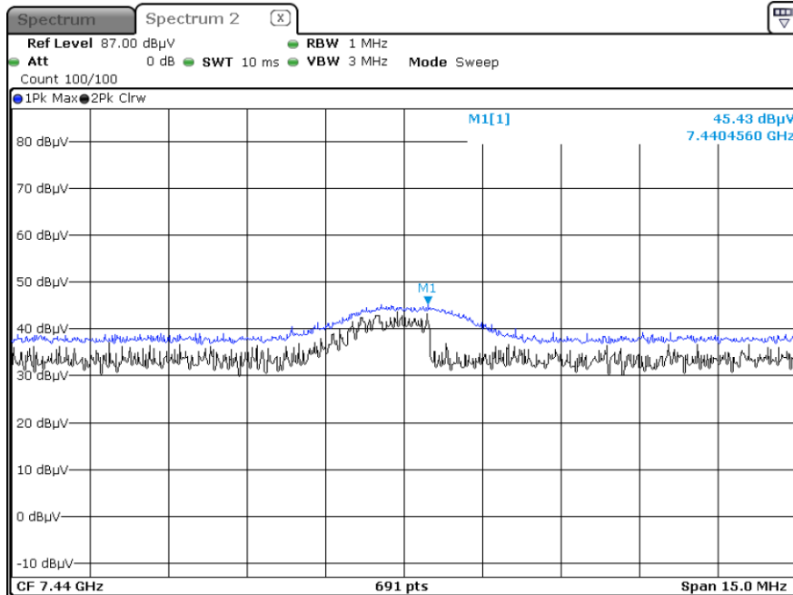
Radiated Spurious Emissions plot –Peak & Average Result( \pi/4 DQPSK, Ch.78 3rd Harmonic, Y-H)
