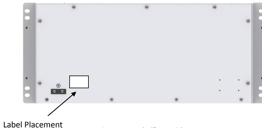
Figure 2 DU shelf rear side
