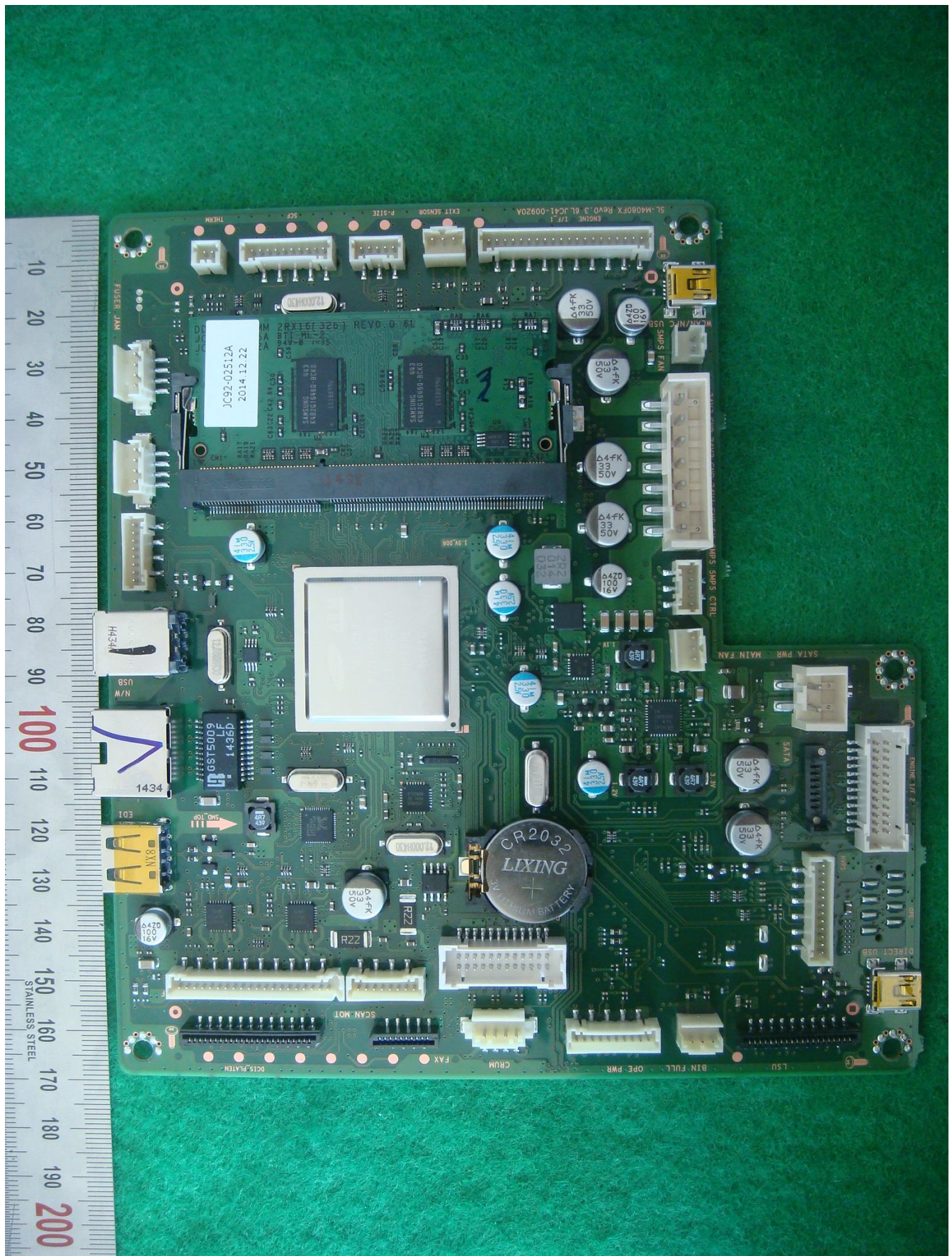
Photograph 3: Internal – Main-board, FRONT view
