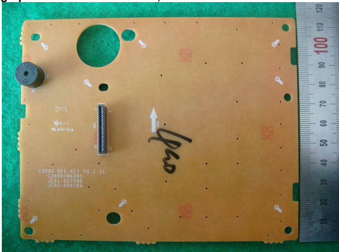
Photograph 19: Internal – OPE KEY, REAR view
