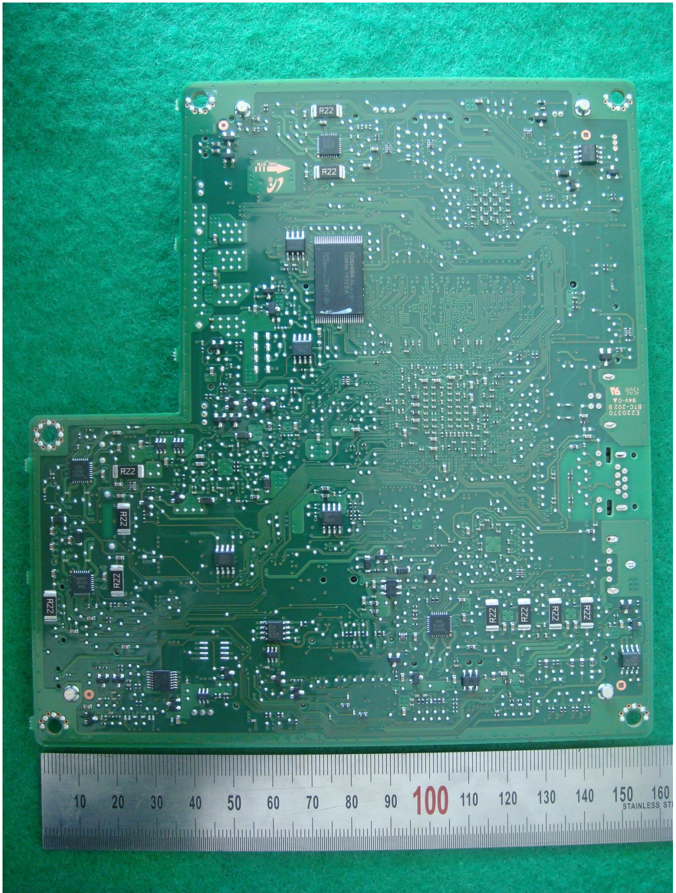
Photograph 5: Internal – Main-board, REAR view
