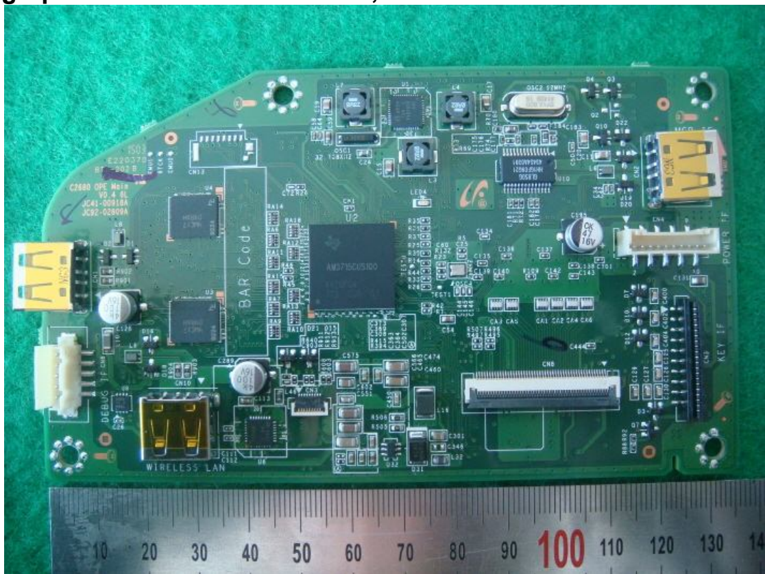
Photograph 16: Internal – OPE MAIN, FRONT view
