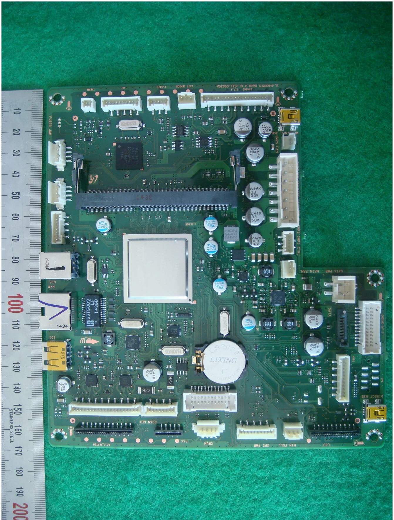
Photograph 4: Internal – Main-board(RAM removed), FRONT view
