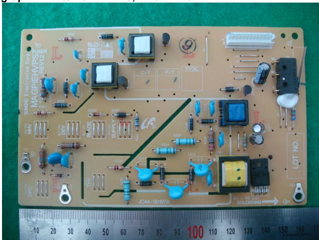
Photograph 14: Internal – HVPS, FRONT view
