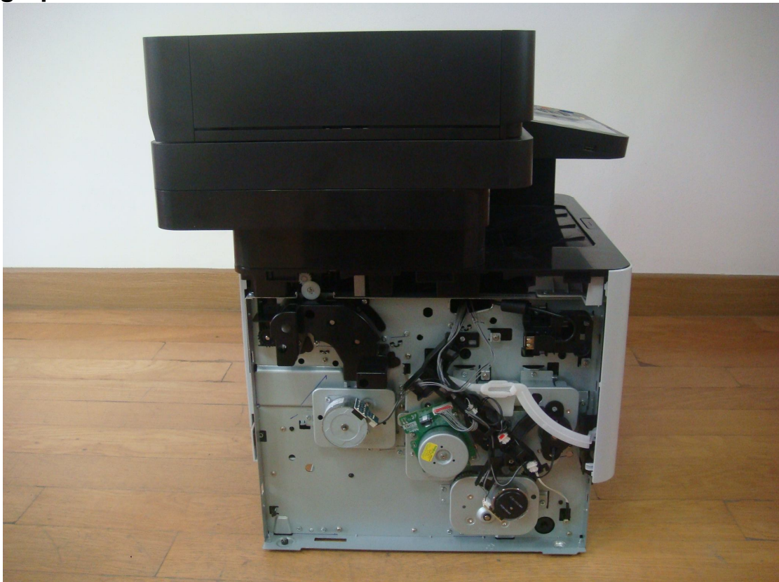
Photograph 2: Cover removed – LEFT VIEW
