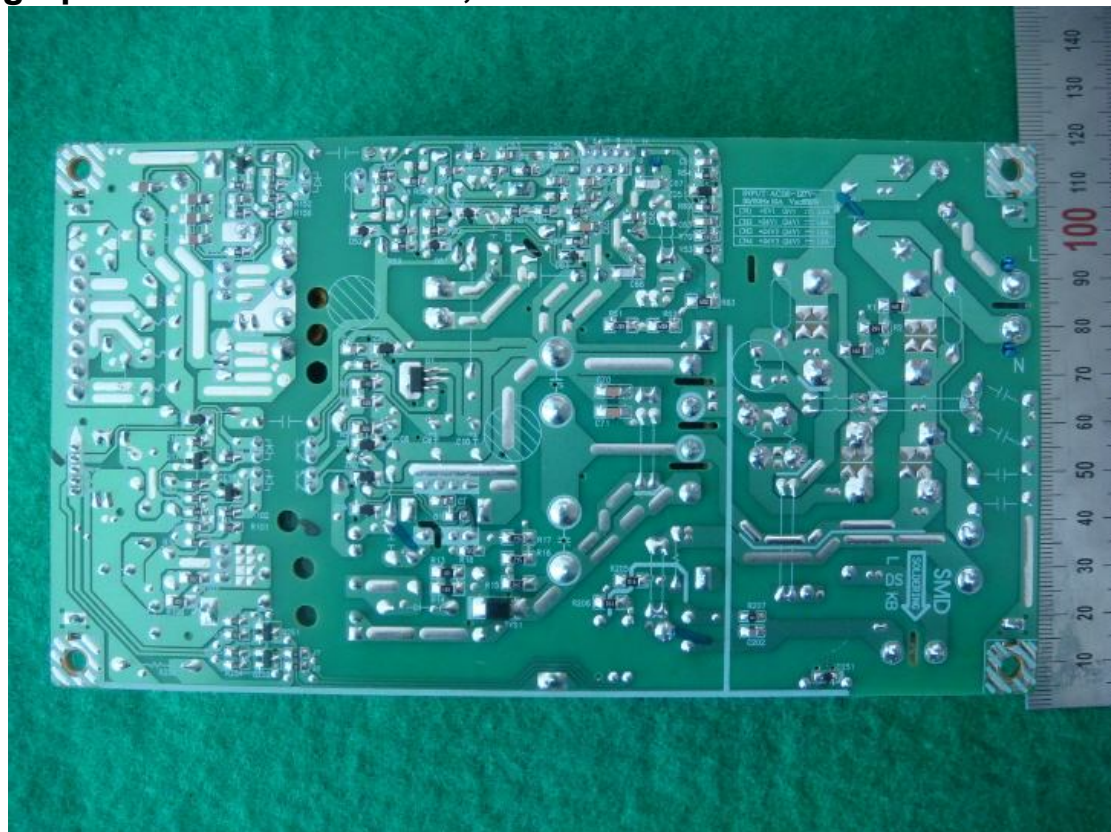
Photograph 13: Internal – SMPS, REAR view
