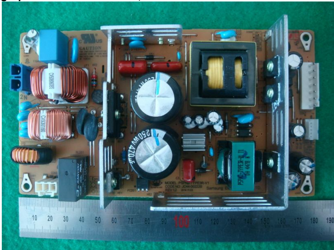
Photograph 12: Internal – SMPS, FRONT view
