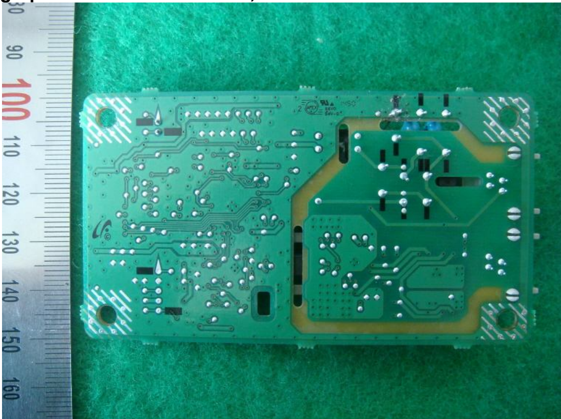
Photograph 11: Internal – MODEM, REAR view
