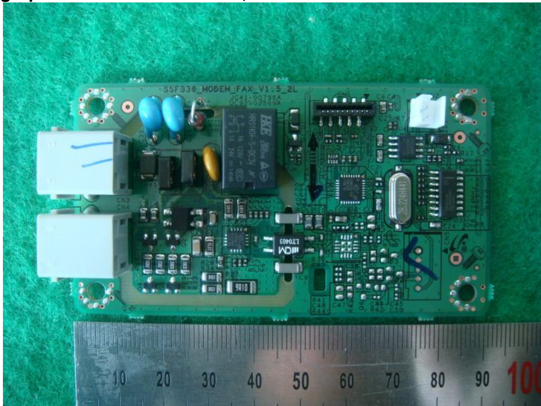
Photograph 10: Internal – MODEM, FRONT view
