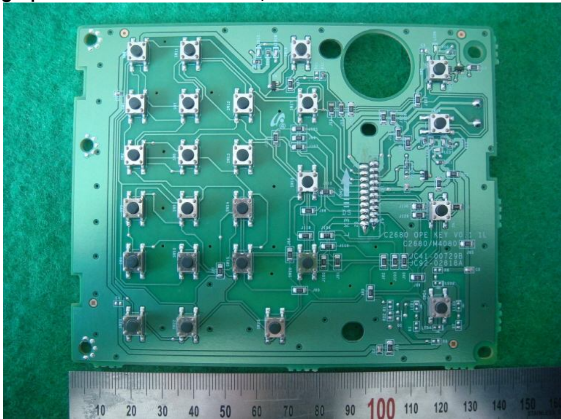
Photograph 18: Internal – OPE KEY, FRONT view
