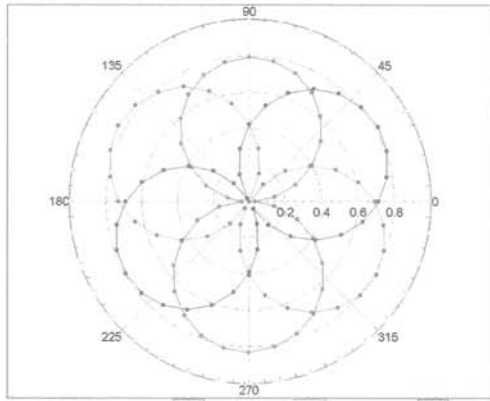
f=600 MHz,TEM
