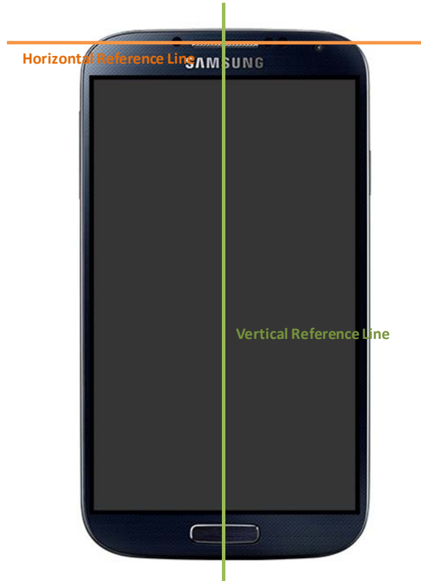
SAR Test Setup Photo 11 – DUT Reference Lines
