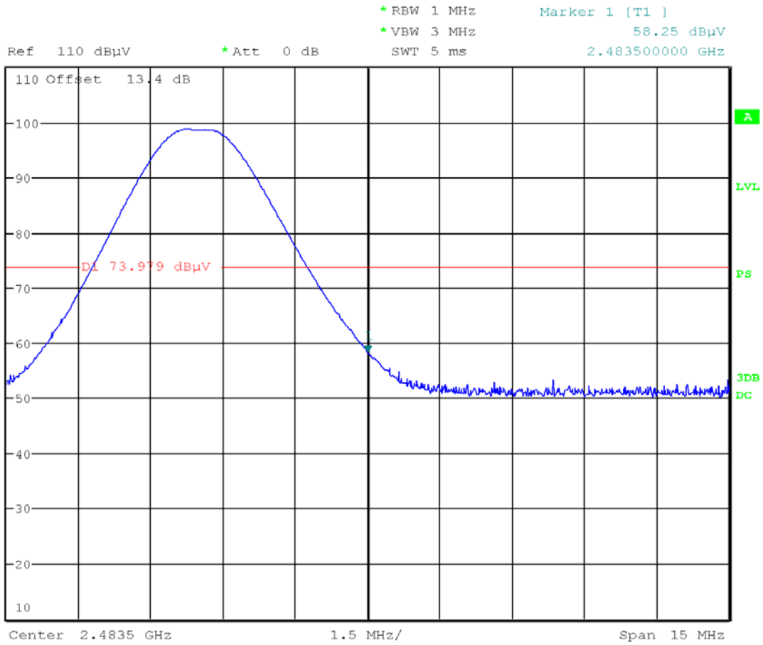
Plot 6-19. Radiated Restricted Upper Band Edge Measurement (Peak)
