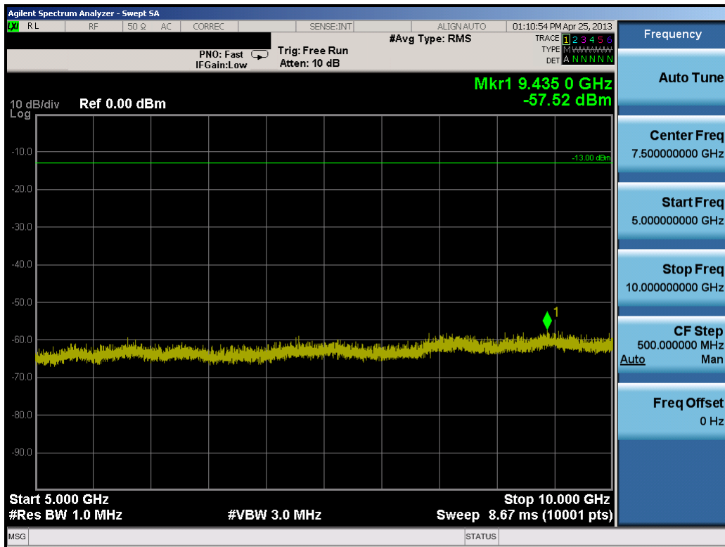
Plot 8-27. Conducted Spurious Plot (10.0MHz QPSK – RB Size 1, RB Offset 0 – Mid Channel)
