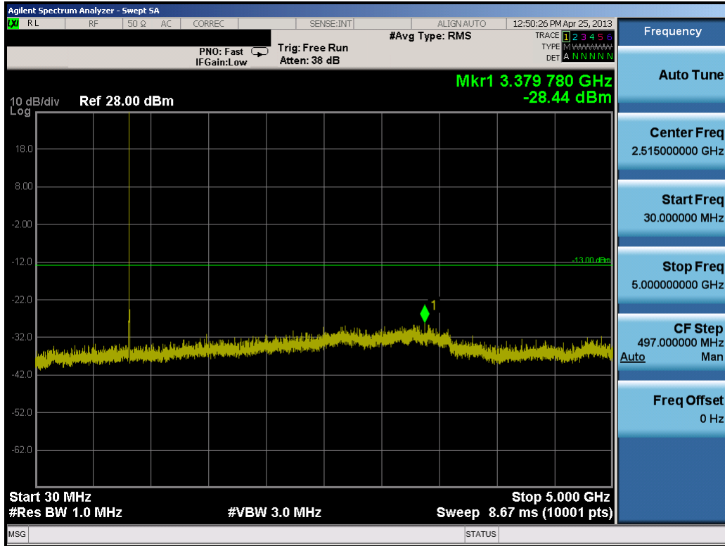
Plot 8-6. Conducted Spurious Plot (3.0MHz QPSK – RB Size 1, RB Offset 0 – Mid Channel)
