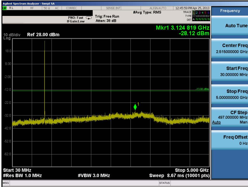
Plot 8-8. Conducted Spurious Plot (3.0MHz QPSK – RB Size 1, RB Offset 0 – High Channel)
