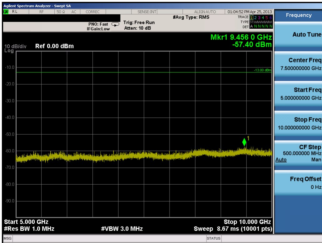
Plot 8-25. Conducted Spurious Plot (10.0MHz QPSK – RB Size 1, RB Offset 0 – Low Channel)
