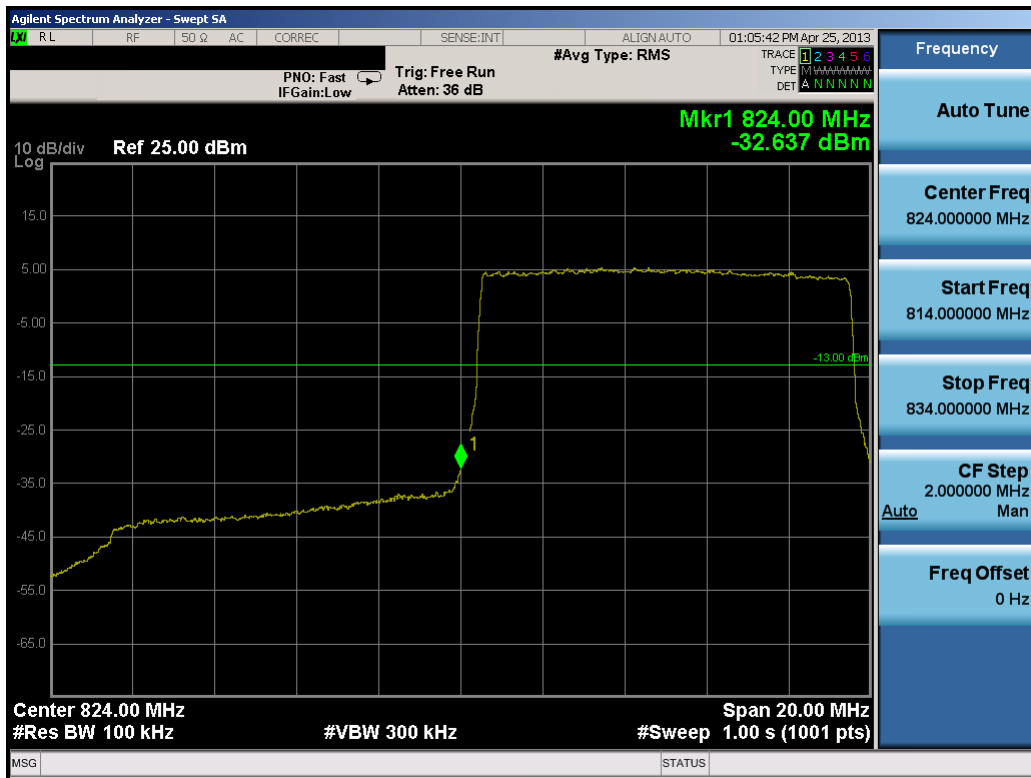
Plot 8-21. Lower Band Edge Plot (10.0MHz QPSK – RB Size 50)
