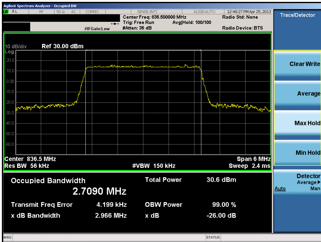
Plot 8-3. Occupied Bandwidth Plot (3.0MHz 16-QAM – RB Size 15)
