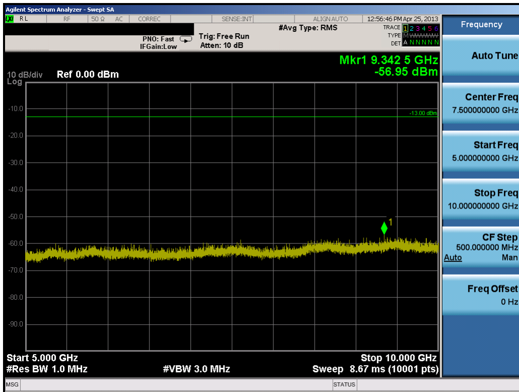
Plot 8-15. Conducted Spurious Plot (5.0MHz QPSK – RB Size 1, RB Offset 0 – Low Channel)
