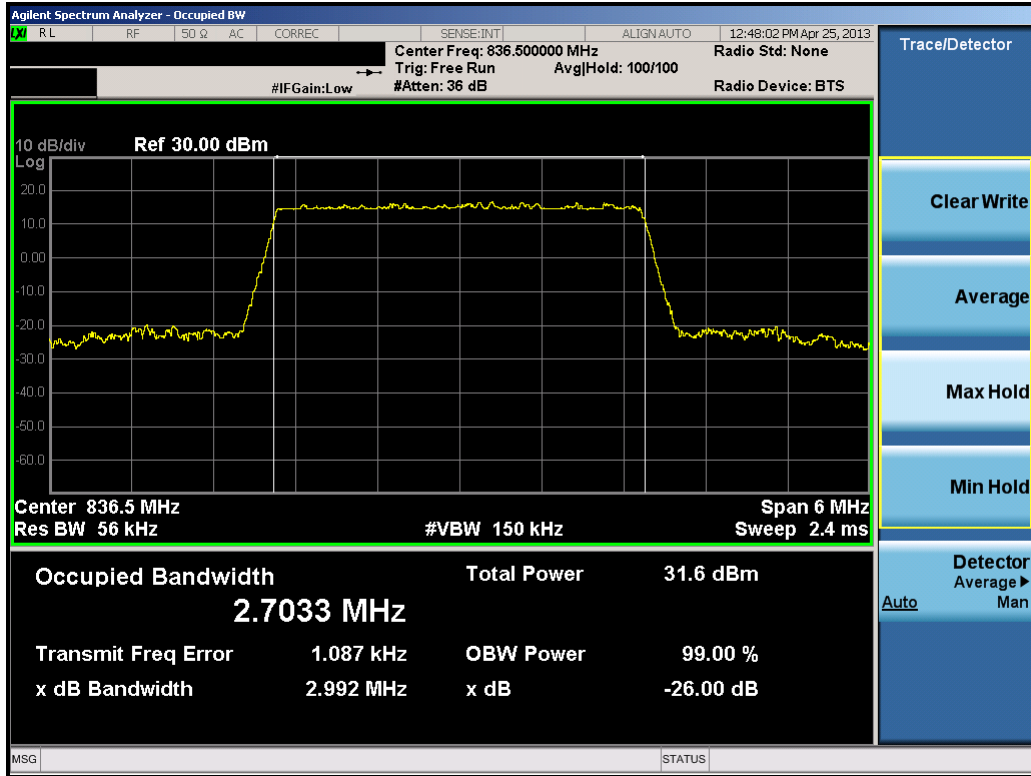
Plot 8-2. Occupied Bandwidth Plot (3.0MHz QPSK – RB Size 15)
