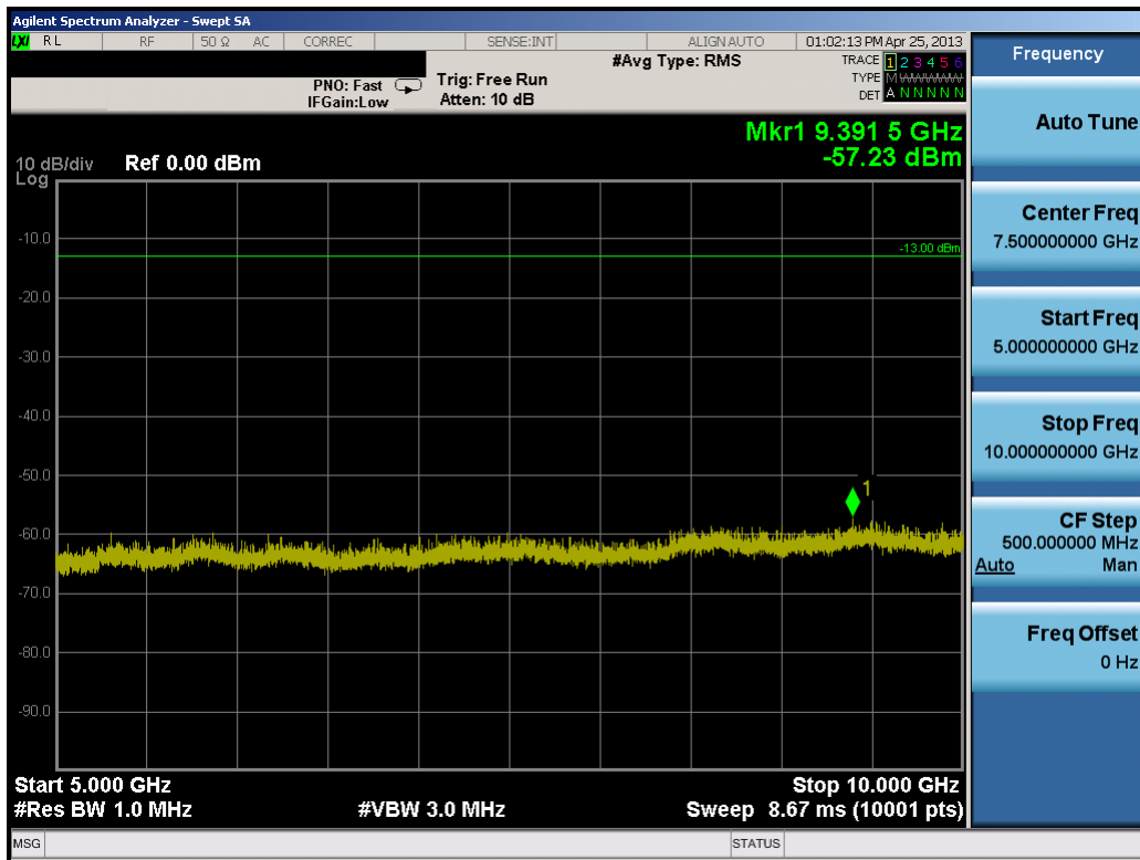
Plot 8-19. Conducted Spurious Plot (5.0MHz QPSK – RB Size 1, RB Offset 0 – High Channel)
