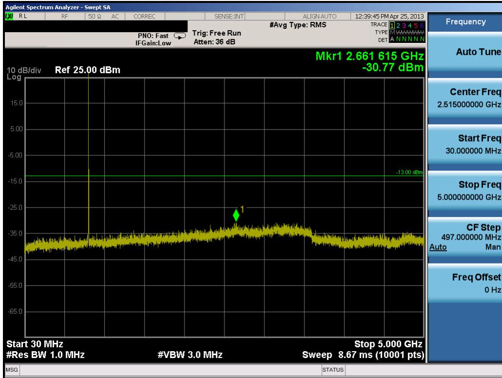
Plot 8-4. Conducted Spurious Plot (3.0MHz QPSK – RB Size 1, RB Offset 0 – Low Channel)
