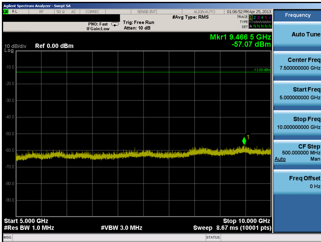
Plot 8-29. Conducted Spurious Plot (10.0MHz QPSK – RB Size 1, RB Offset 0 – High Channel)
