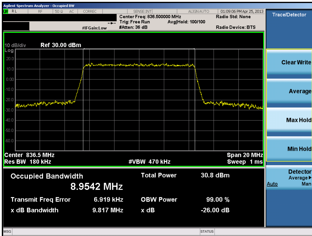
Plot 8-23. Occupied Bandwidth Plot (10.0MHz 16-QAM – RB Size 50)
