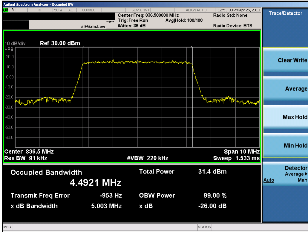
Plot 8-12. Occupied Bandwidth Plot (5.0MHz QPSK – RB Size 25)
