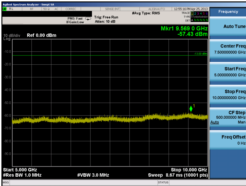
Plot 8-17. Conducted Spurious Plot (5.0MHz QPSK – RB Size 1, RB Offset 0 – Mid Channel)
