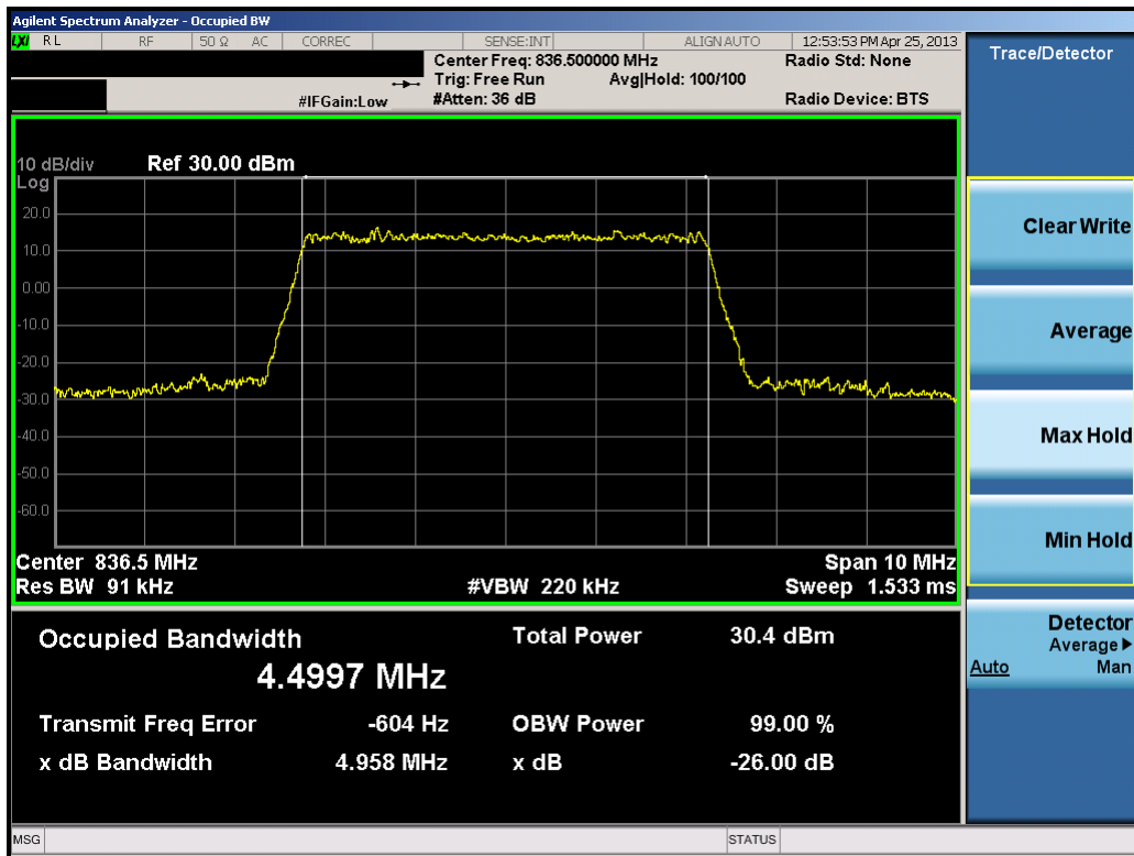
Plot 8-13. Occupied Bandwidth Plot (5.0MHz 16-QAM – RB Size 25)
