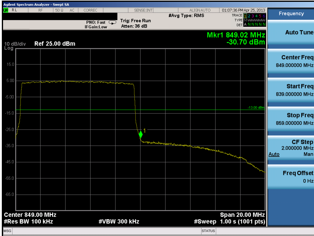
Plot 8-30. Upper Band Edge Plot (10.0MHz QPSK – RB Size 50)
