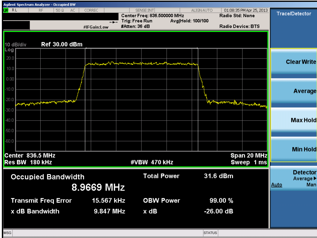
Plot 8-22. Occupied Bandwidth Plot (10.0MHz QPSK – RB Size 50)
