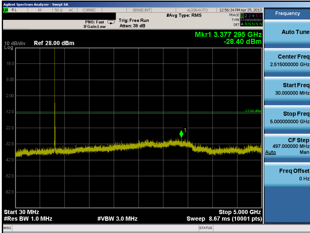
Plot 8-14. Conducted Spurious Plot (5.0MHz QPSK – RB Size 1, RB Offset 0 – Low Channel)
