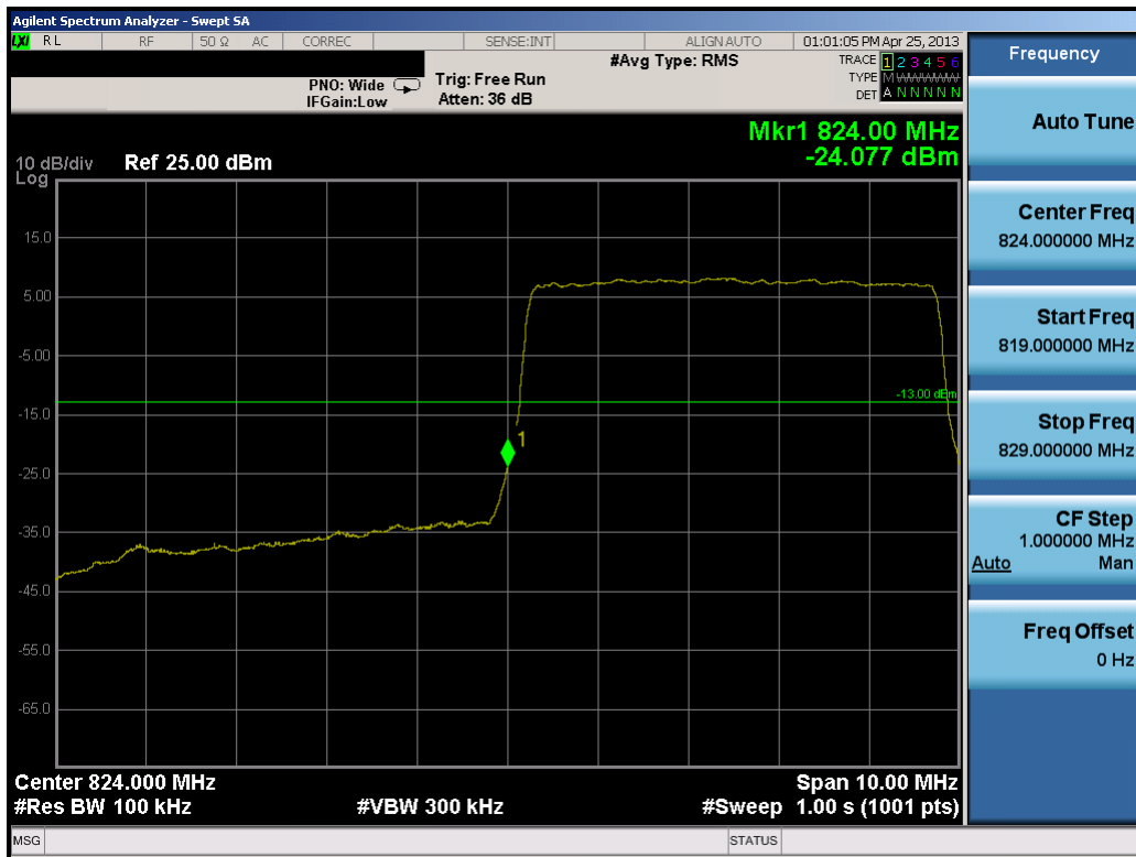
Plot 8-11. Lower Band Edge Plot (5.0MHz QPSK – RB Size 25)
