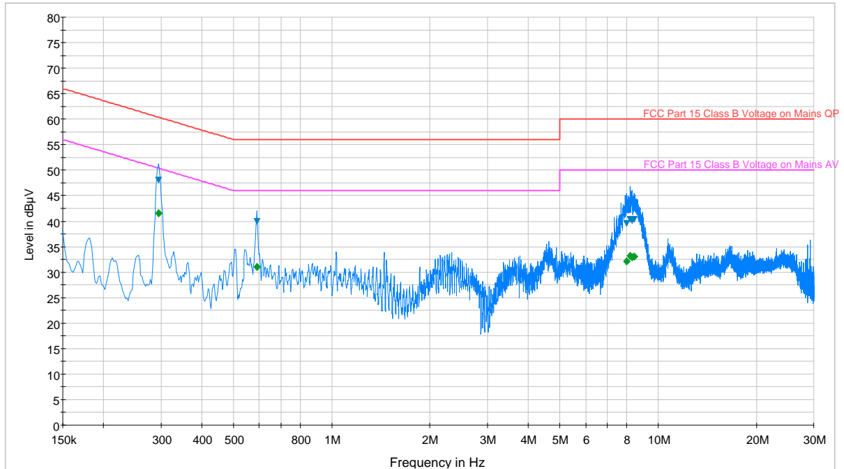
Plot 6-87. Line Conducted Plot with 802.11a UNII Band 2 (N)
