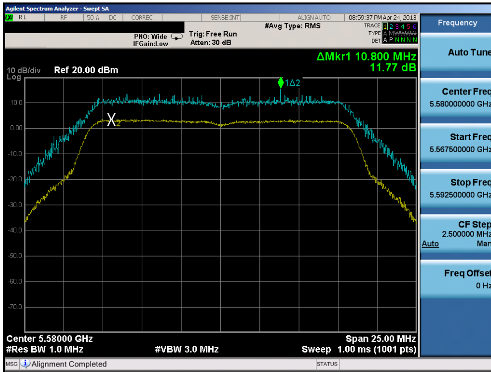
Plot 6-61. Peak Excursion Ratio Plot (802.11a)
