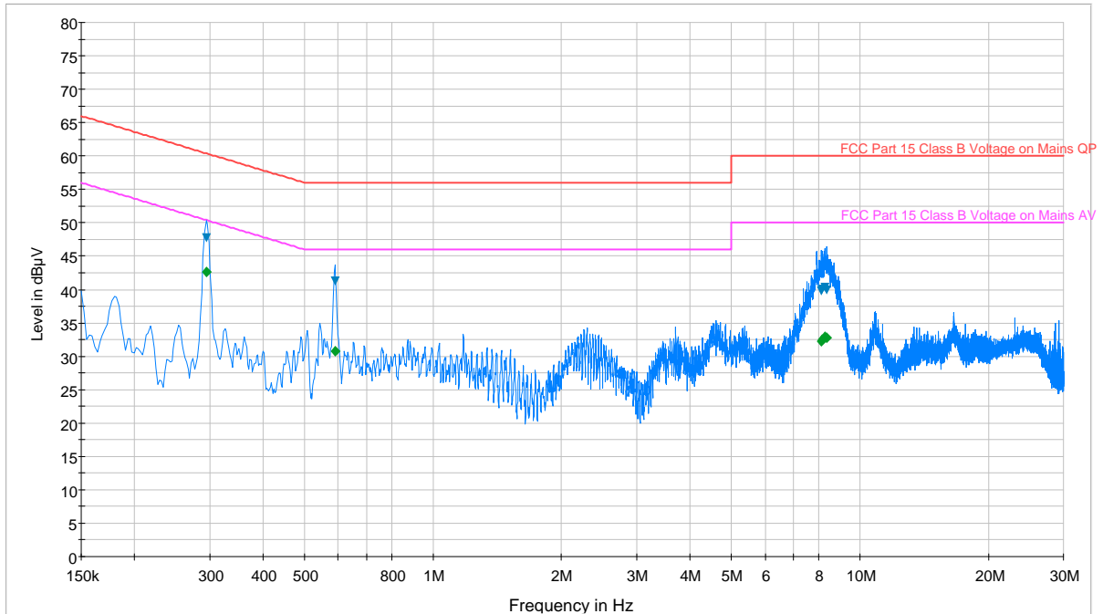
Plot 6-85. Line Conducted Plot with 802.11a UNII Band 1 (N)
