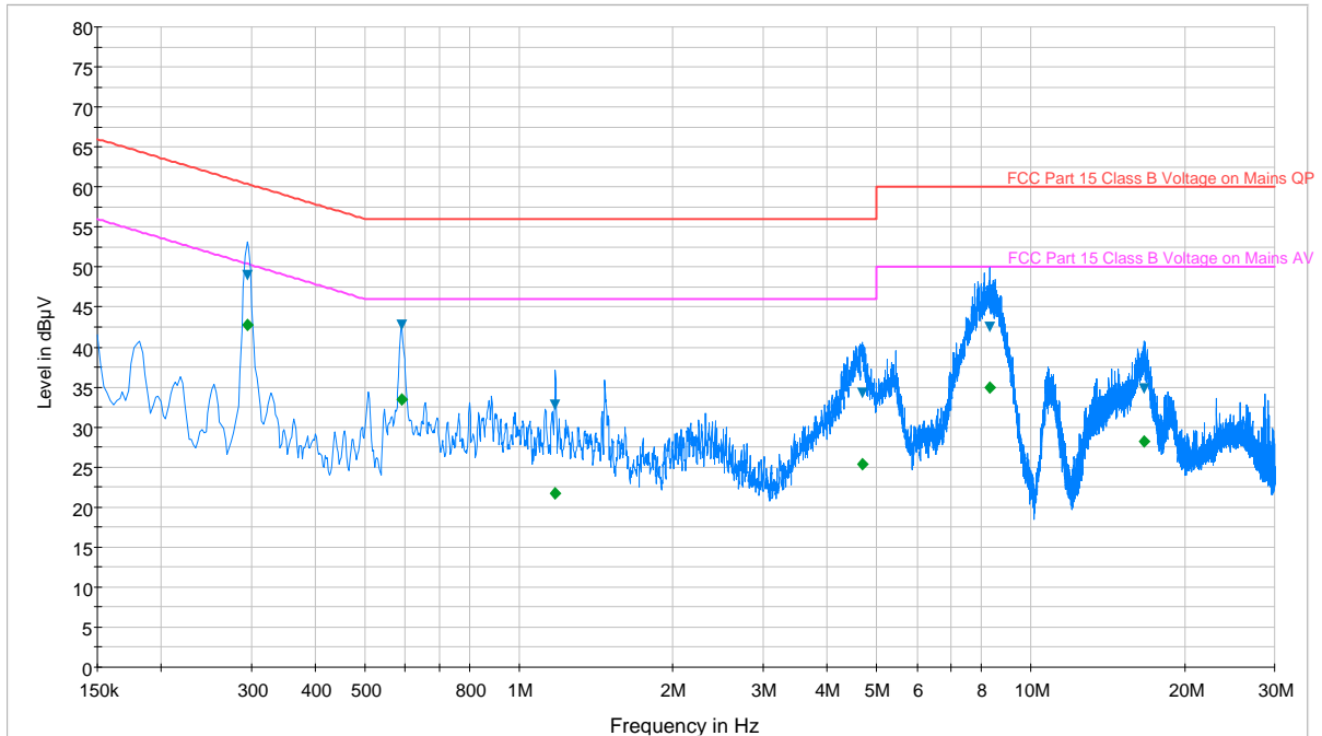
Plot 6-84. Line Conducted Plot with 802.11a UNII Band 1 (L1)
