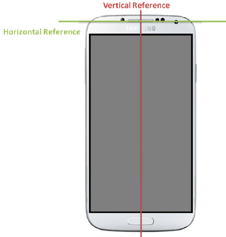
SAR Test Setup Photo 11: DUT Horizontal and Vertical Reference Lines
