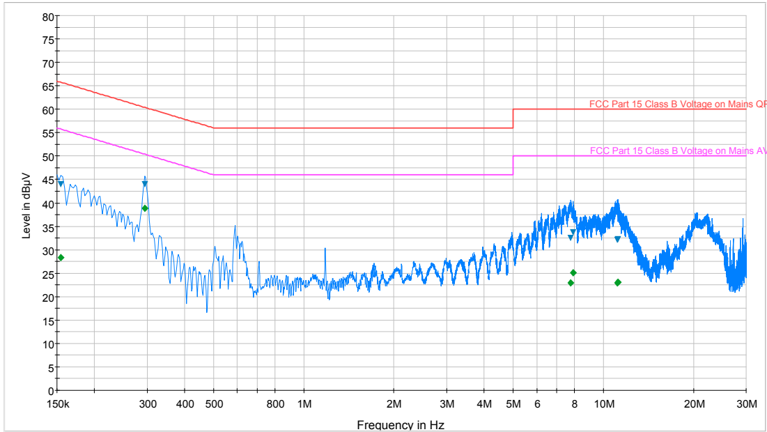
Plot 6-18. Line Conducted Plot with Bluetooth LE (N)
