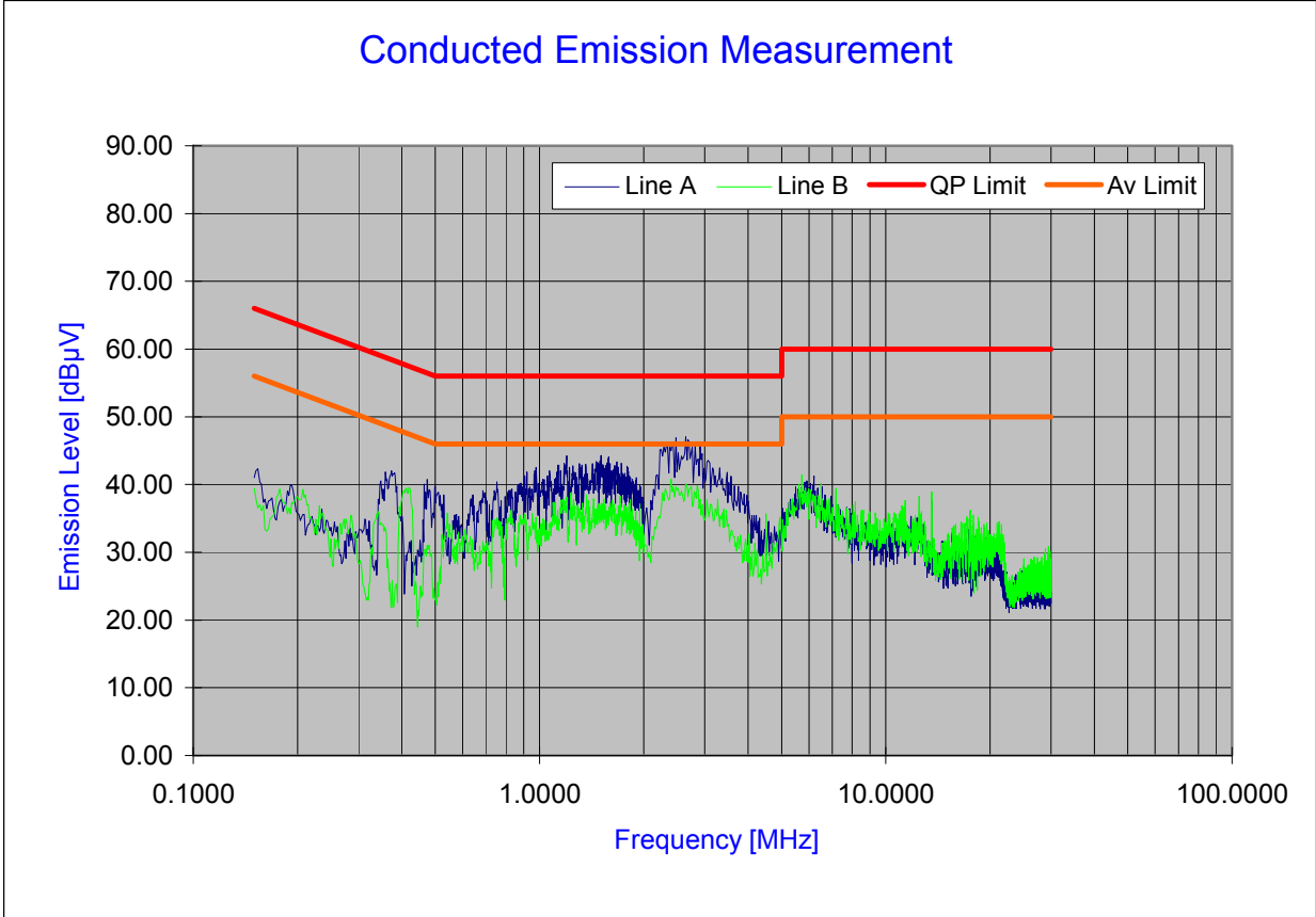
Plot 6-17. Line Conducted Plot with Bluetooth LE
