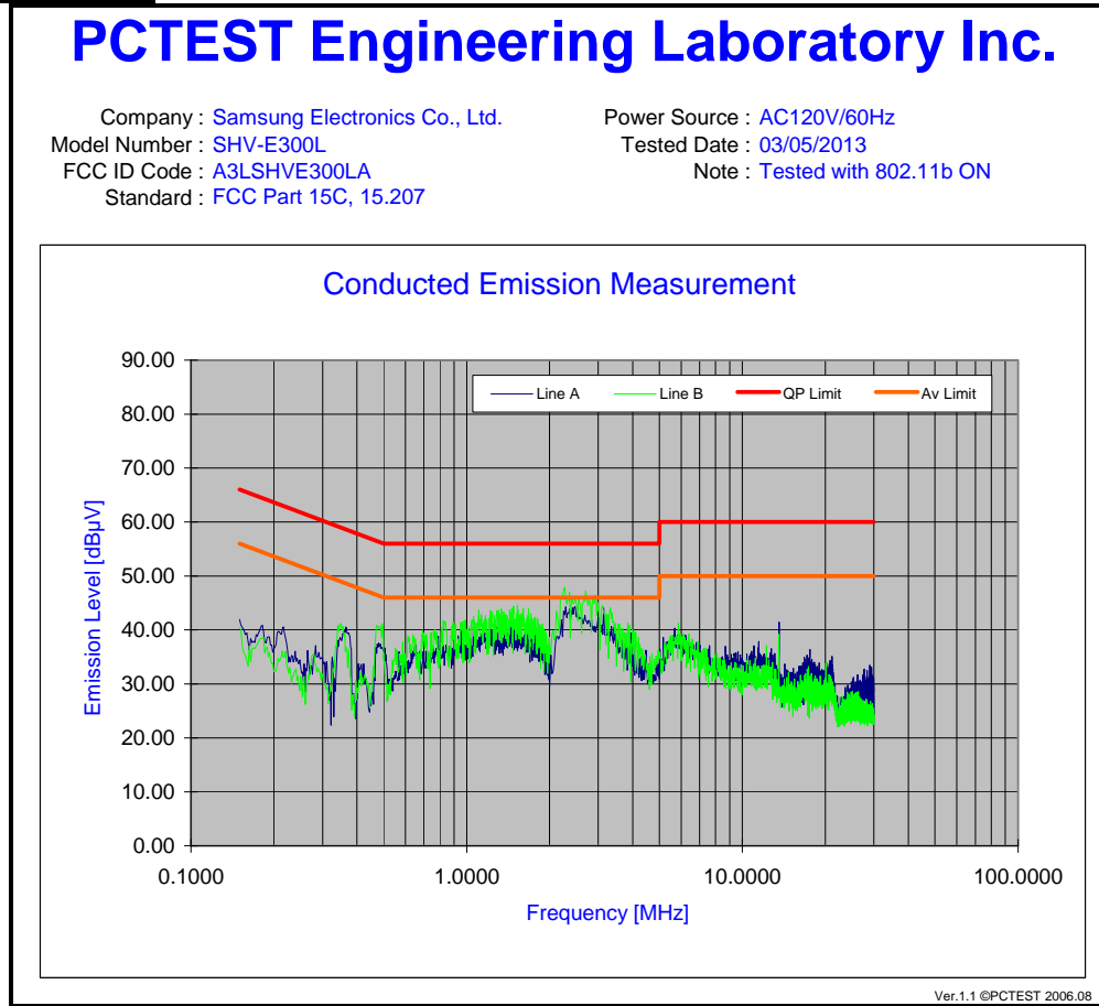
Plot 6-67. Line Conducted Plot with 802.11b
