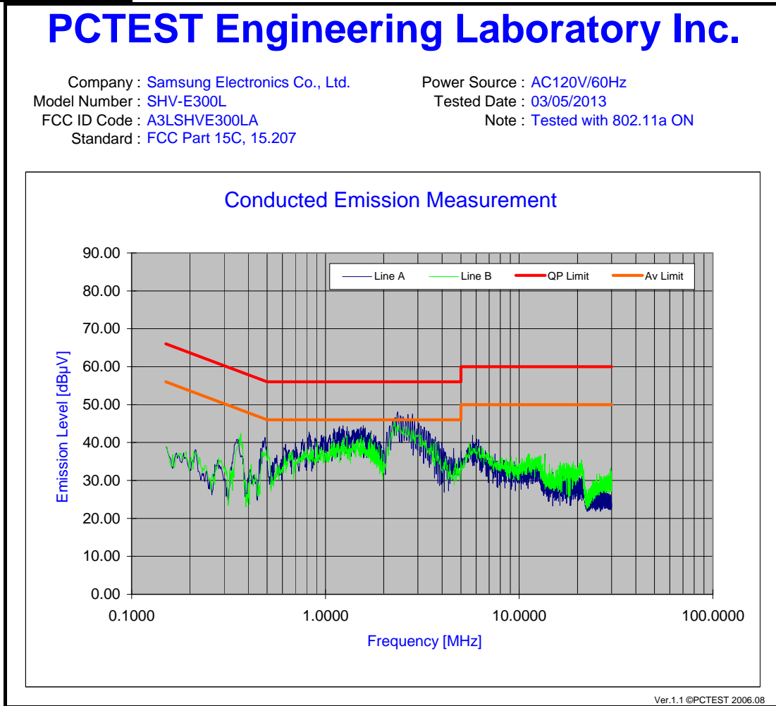
Plot 6-68. Line Conducted Plot with 802.11a
