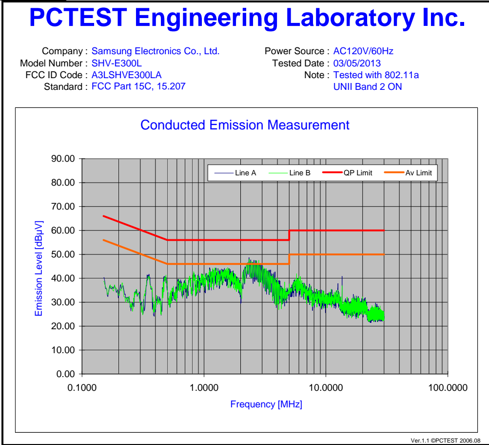
Plot 6-82. Line Conducted Plot with 802.11a UNII Band 2
