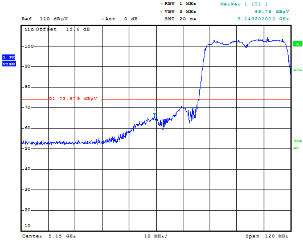
Plot 6-69. Radiated Restricted Lower Band Edge Plot (Peak – UNII Band 1)
