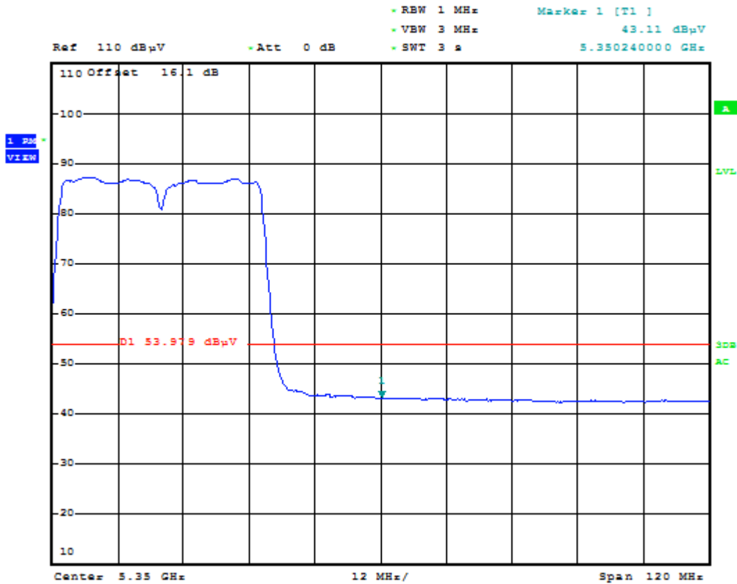
Plot 6-70. Radiated Restricted Upper Band Edge Plot (Average – UNII Band 2)
