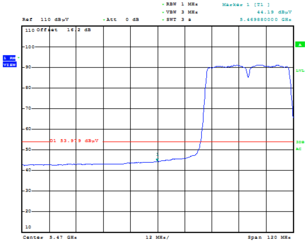
Plot 6-72. Radiated Restricted Lower Band Edge Plot (Average – UNII Band 3)
