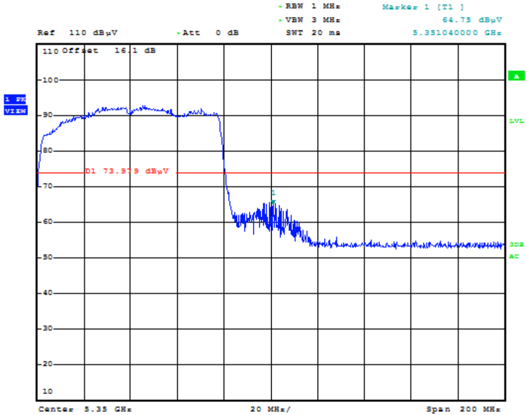
Plot 6-78. Radiated Restricted Upper Band Edge Plot (Peak – UNII Band 2)
