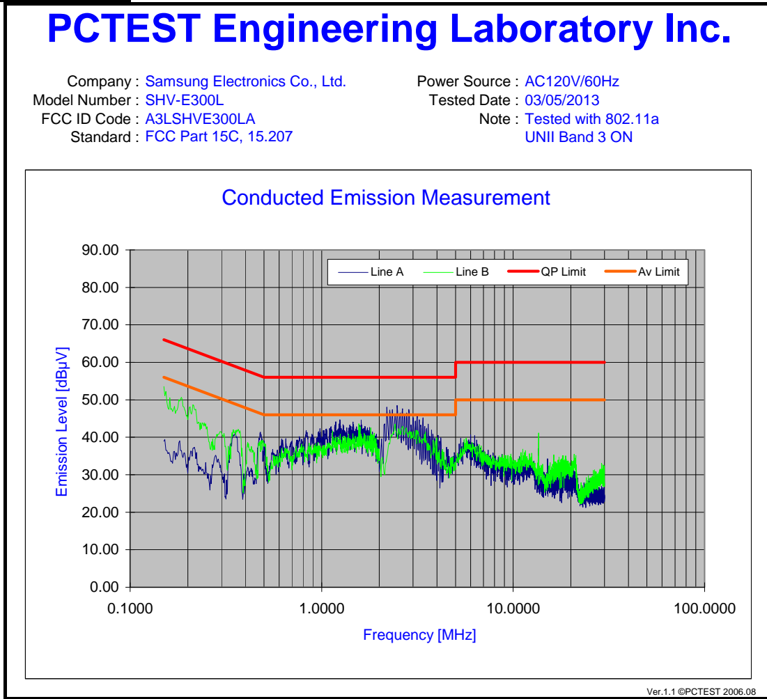
Plot 6-83. Line Conducted Plot with 802.11a UNII Band 3
