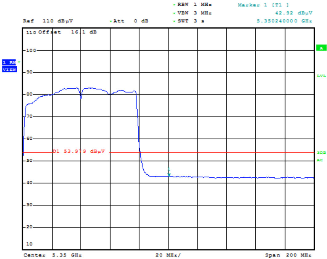
Plot 6-77. Radiated Restricted Upper Band Edge Plot (Average – UNII Band 2)
