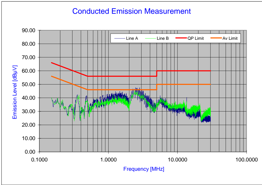
Plot 6-81. Line Conducted Plot with 802.11a UNII Band 1
