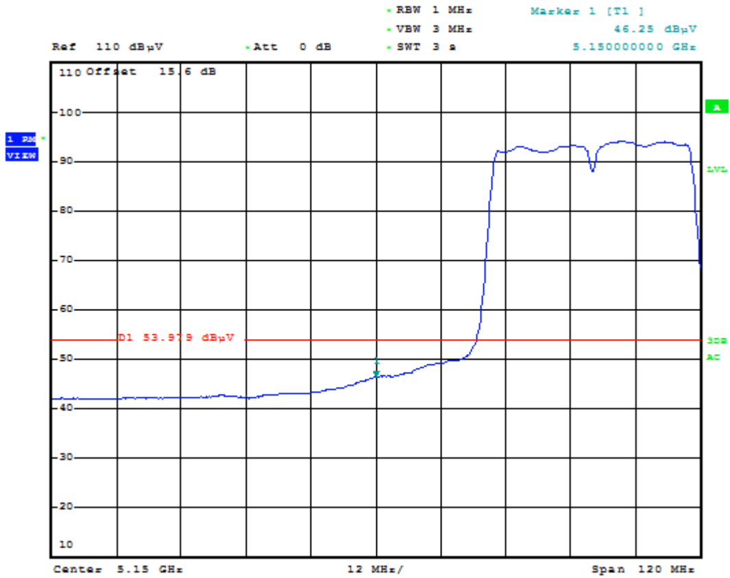
Plot 6-68. Radiated Restricted Lower Band Edge Plot (Average – UNII Band 1)
