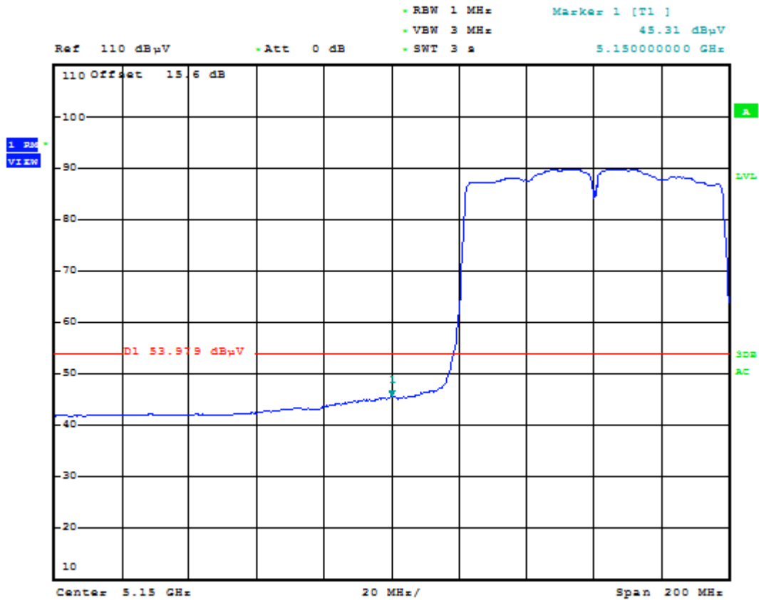
Plot 6-75. Radiated Restricted Lower Band Edge Plot (Average – UNII Band 1)
