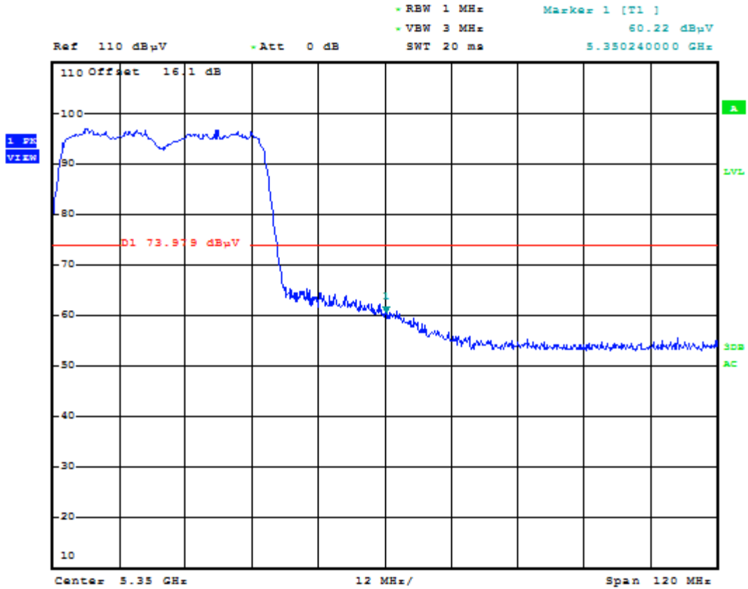
Plot 6-71. Radiated Restricted Upper Band Edge Plot (Peak – UNII Band 2)
