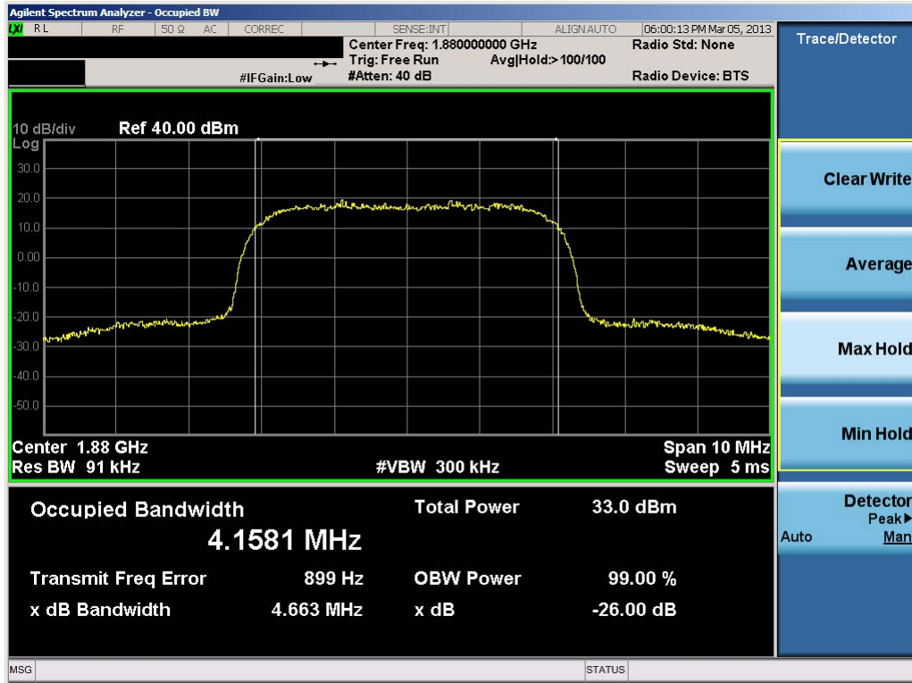
Plot 7-26. Occupied Bandwidth Plot (PCS WCDMA Mode – Ch. 9400)
