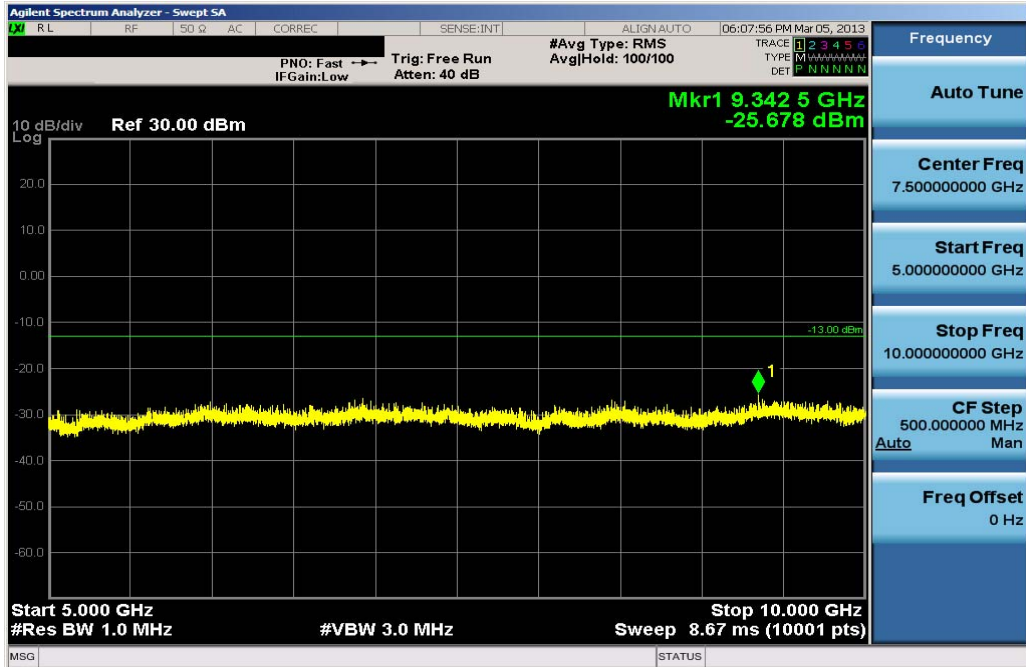
Plot 7-18. Conducted Spurious Plot (Cellular WCDMA Mode – Ch. 4233)
