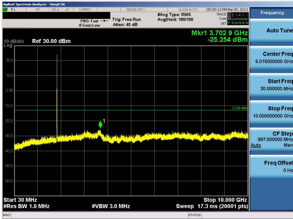
Plot 7-20. Conducted Spurious Plot (PCS WCDMA Mode – Ch. 9262)
