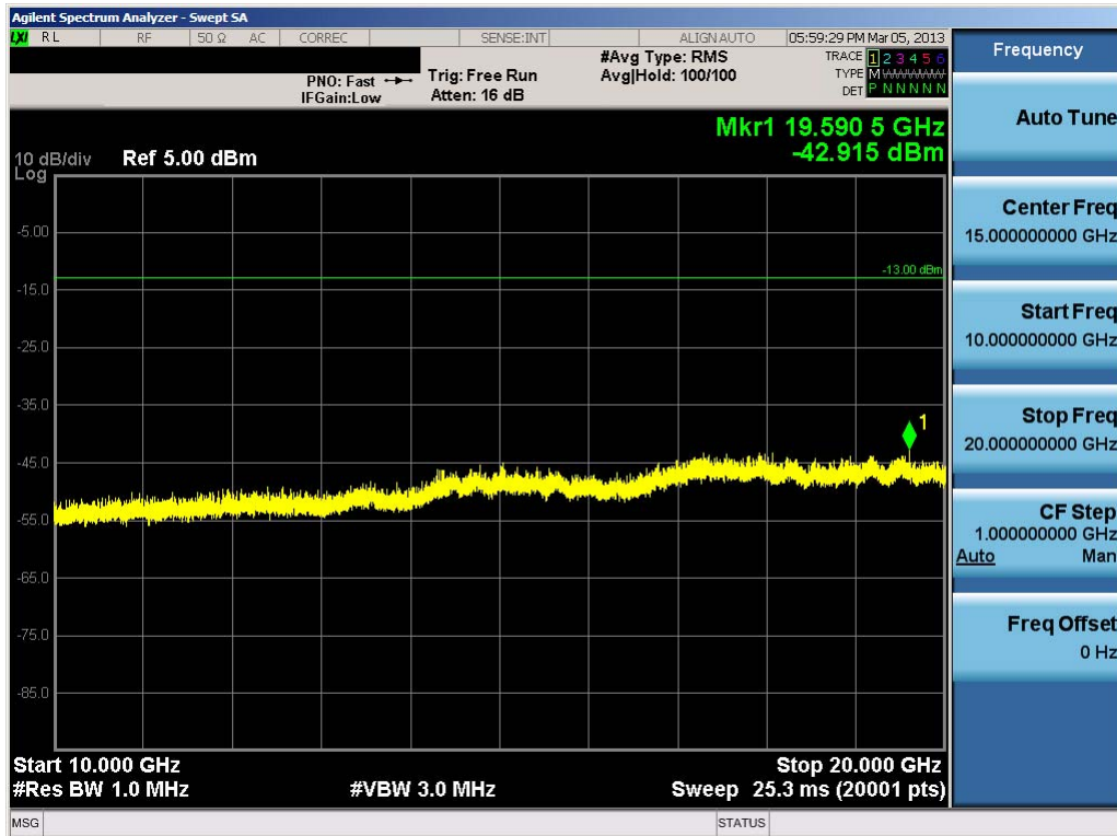
Plot 7-21. Conducted Spurious Plot (PCS WCDMA Mode – Ch. 9262)
