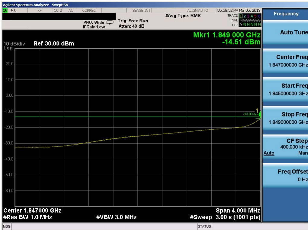
Plot 7-23. 4MHz Span Plot (PCS WCDMA Mode – Ch. 9262)
