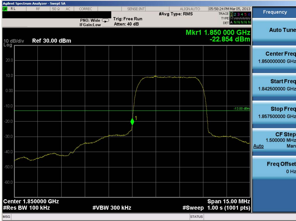
Plot 7-22. Band Edge Plot (PCS WCDMA Mode – Ch. 9262)
