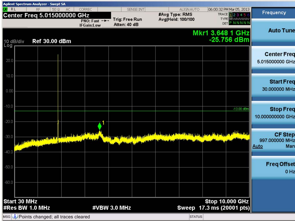
Plot 7-24. Conducted Spurious Plot (PCS WCDMA Mode – Ch. 9400)
