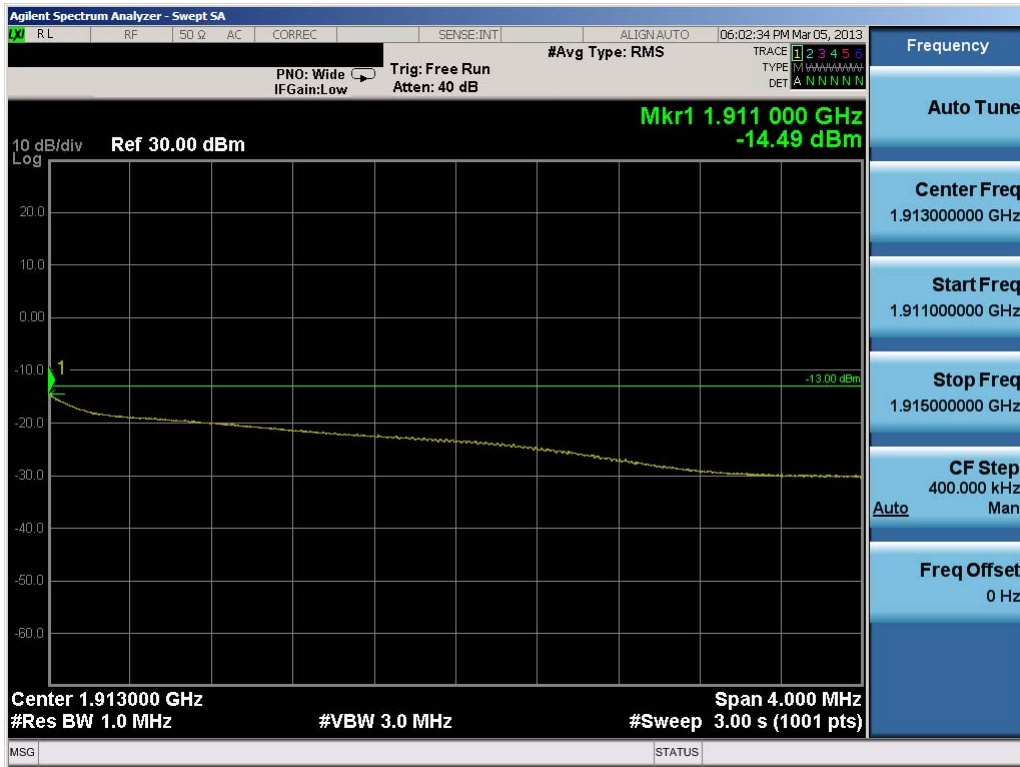
Plot 7-31. 4MHz Span Plot (PCS WCDMA Mode – Ch. 9538)
