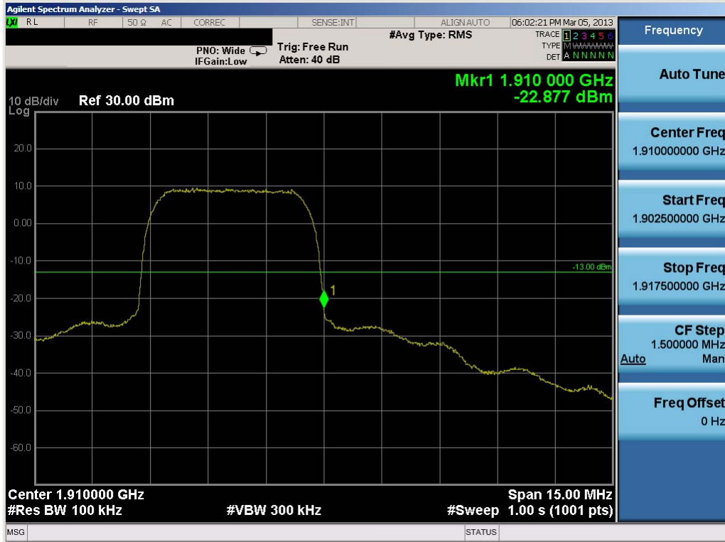
Plot 7-30. Band Edge Plot (PCS WCDMA Mode – Ch. 9538)
