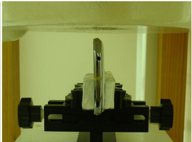
Left Side with Phantom 1 cm Gap
