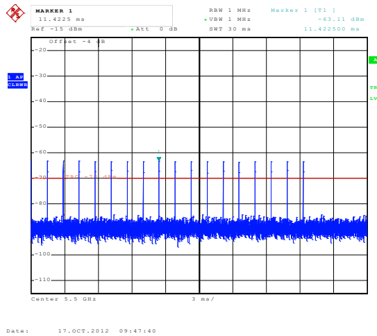
Radar #1 DFS detection threshold level
