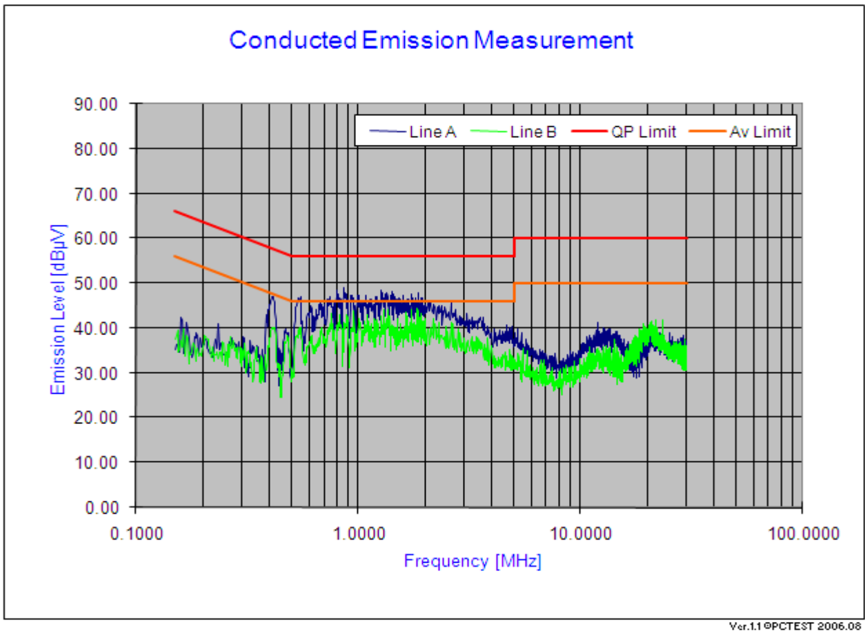
Plot 6-59. Line Conducted Plot with 802.11n (UNII Band 2)
