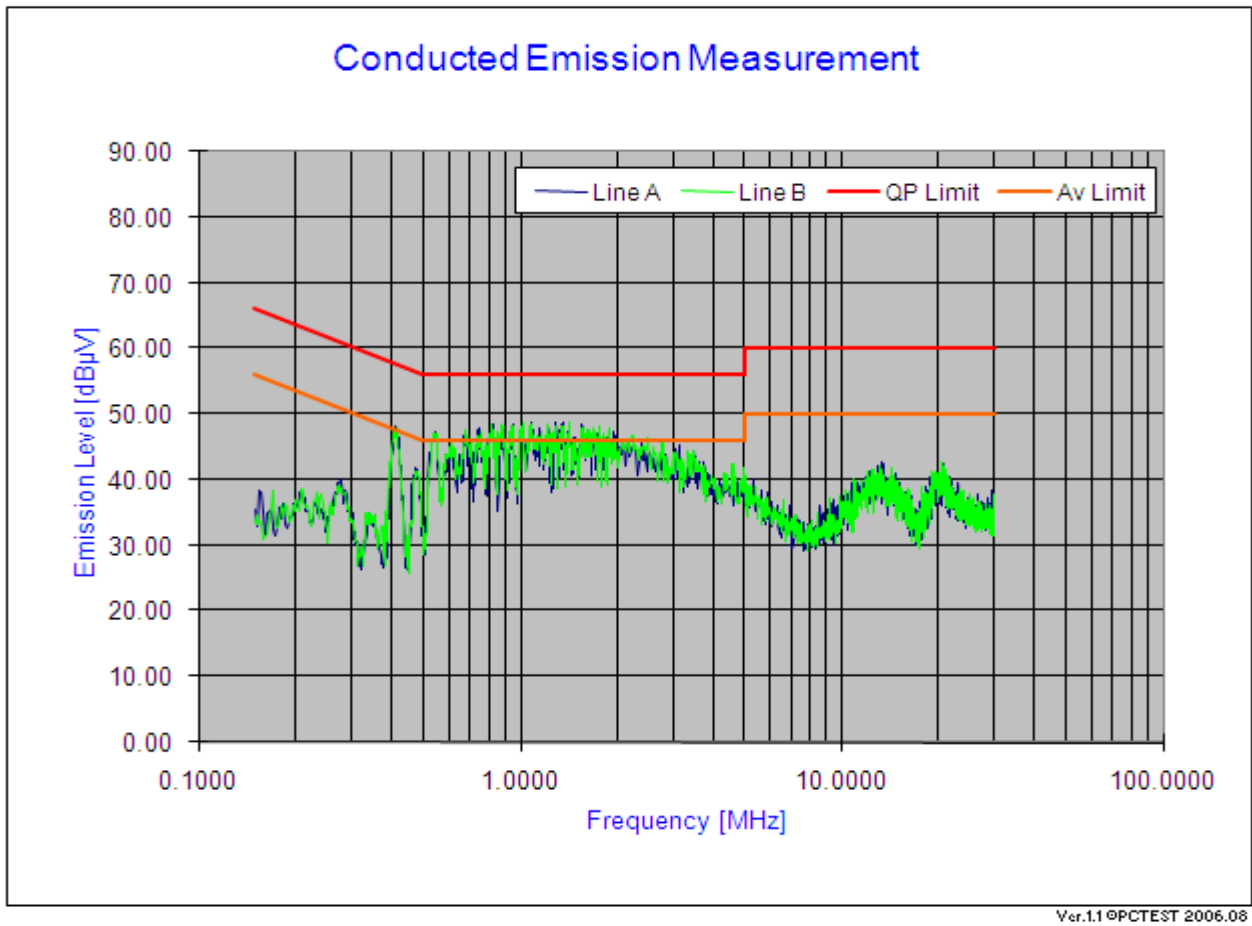
Plot 6-56. Line Conducted Plot with 802.11a (UNII Band 2)
