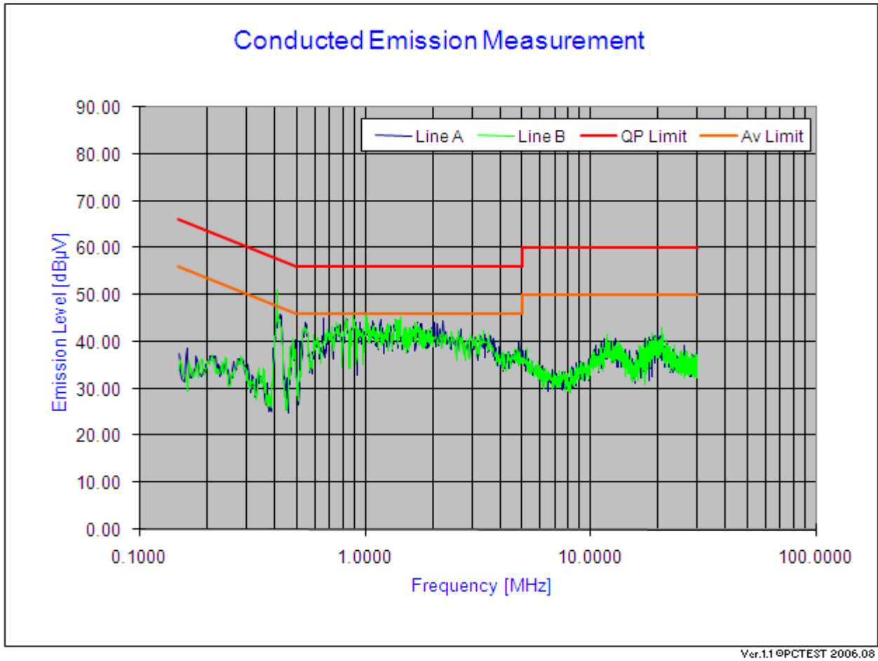
Plot 6-55. Line Conducted Plot with 802.11a (UNII Band 1)
