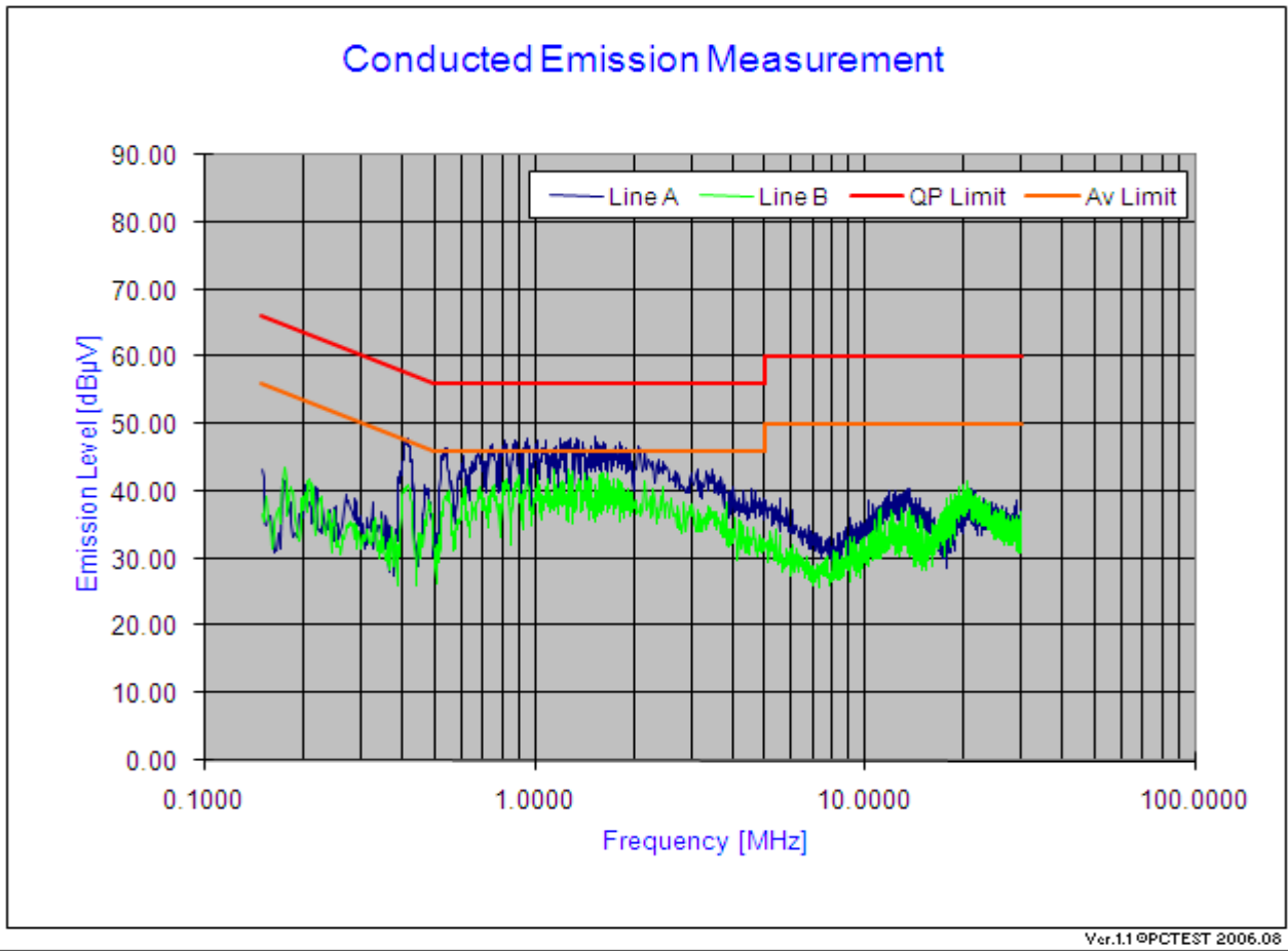
Plot 6-58. Line Conducted Plot with 802.11n (UNII Band 1)
