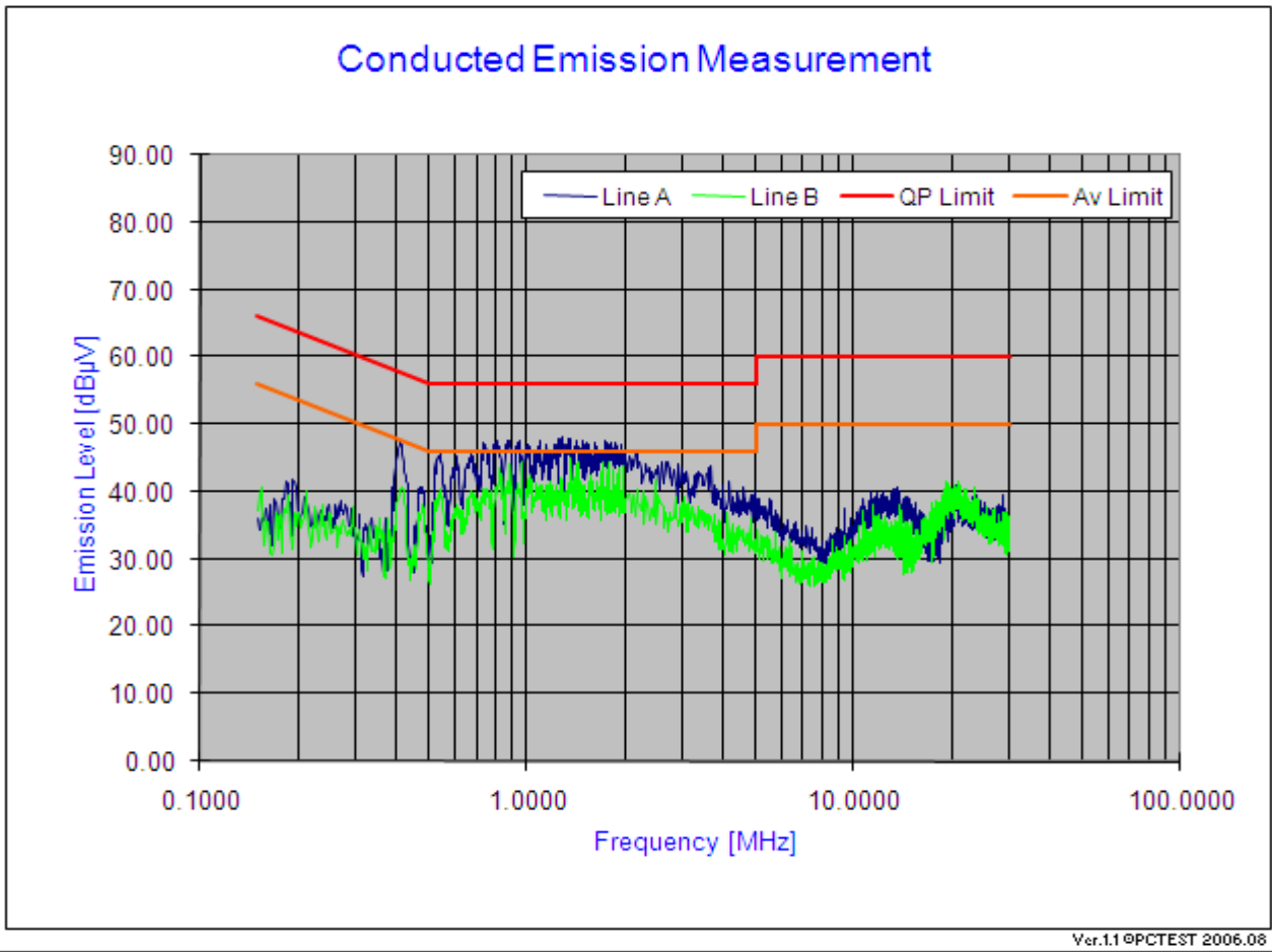
Plot 6-60. Line Conducted Plot with 802.11n (UNII Band 3)
