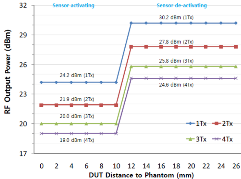
Figure 9-4 GPRS (GMSK) 1900 Back off Power Reduction Graph - Back Side
