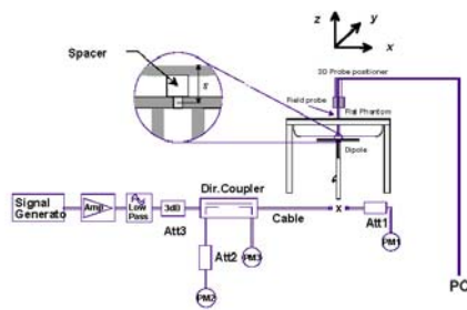
Fig 12-3 System Verification Setup Diagram
