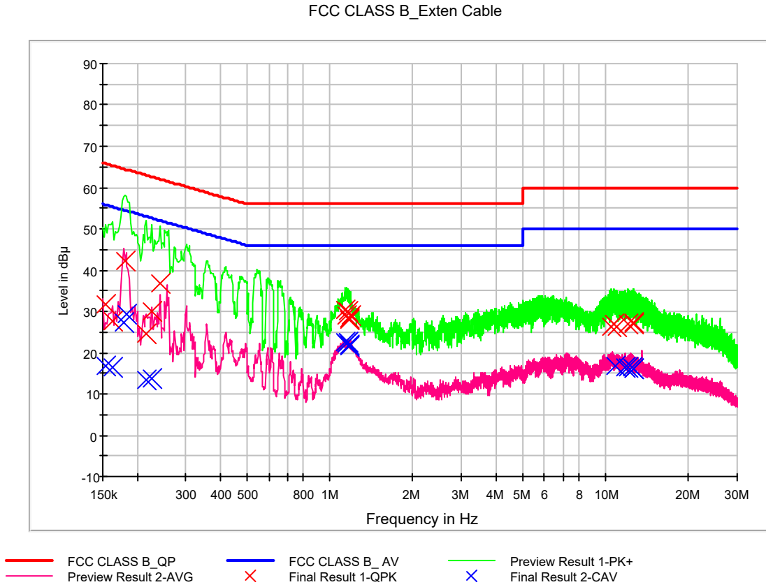
Figure 7: Conducted Emission, Charging & Receiver at WCDMA 850, GSM 850, LTE B5 (Middle CH Idle), Line (L1)
