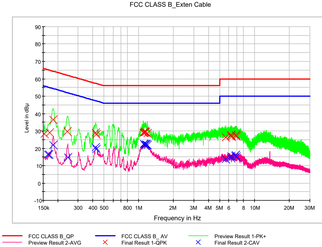
Figure 8: Conducted Emission, Charging & Receiver at WCDMA 850, GSM 850, LTE B5 (Middle CH Idle), Line (N)
