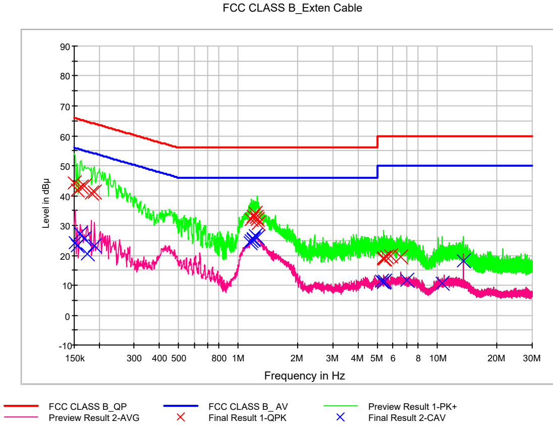
Figure 6: Conducted Emission, Charging & Receiver mode at LTE B12, LTE B17 (Middle CH Idle), Line (N)
