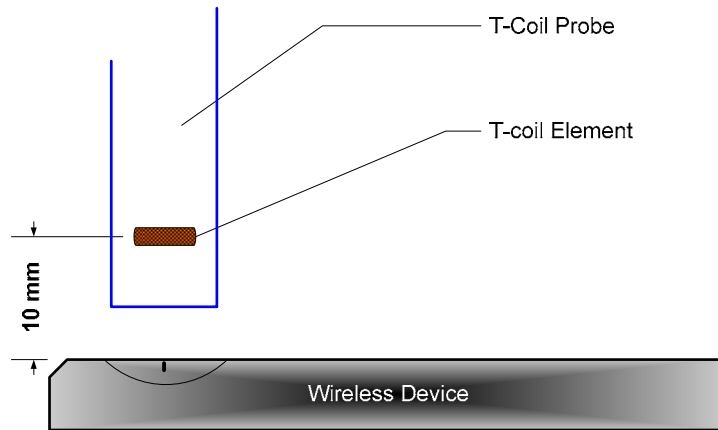
Figure 5-11 Measurement Distance
