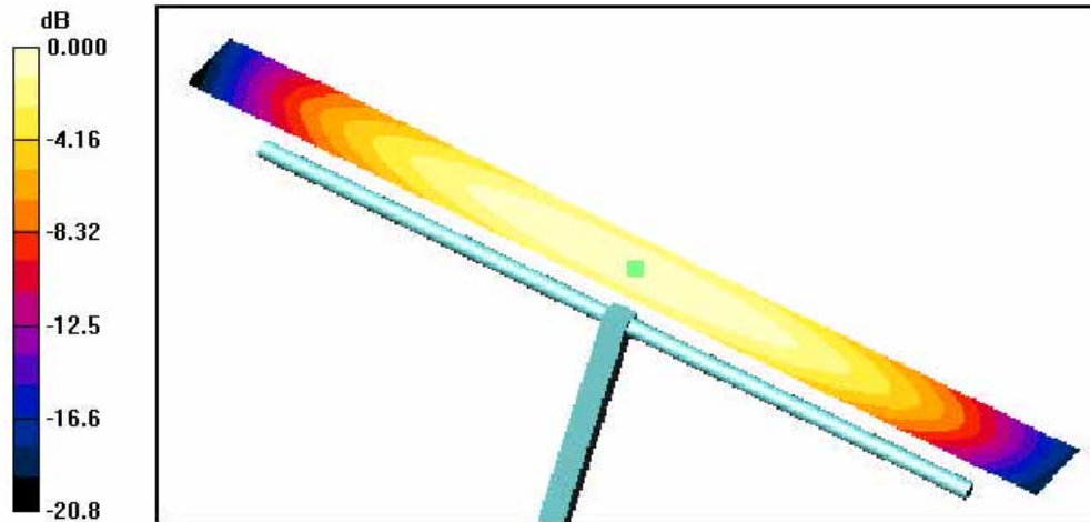
0 dB = 0.505A/m
