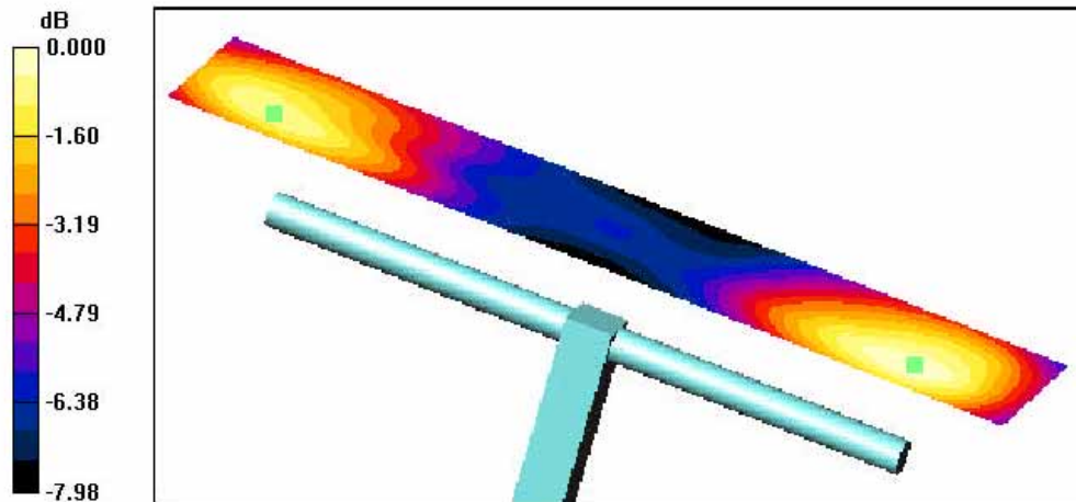
0 dB = 150.3V/m
