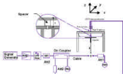
Figure 12.1 Dipole Validation
