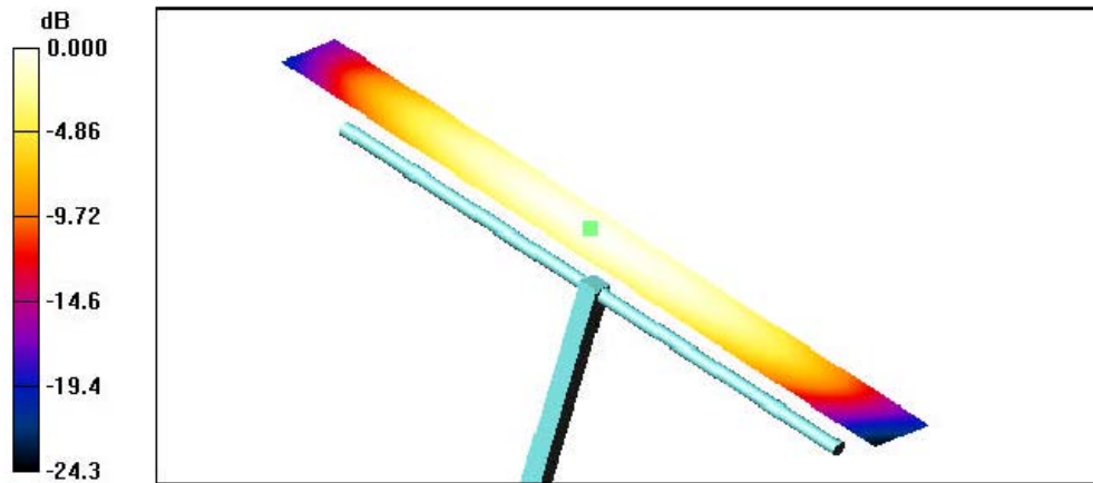
0 dB = 0.468A/m
