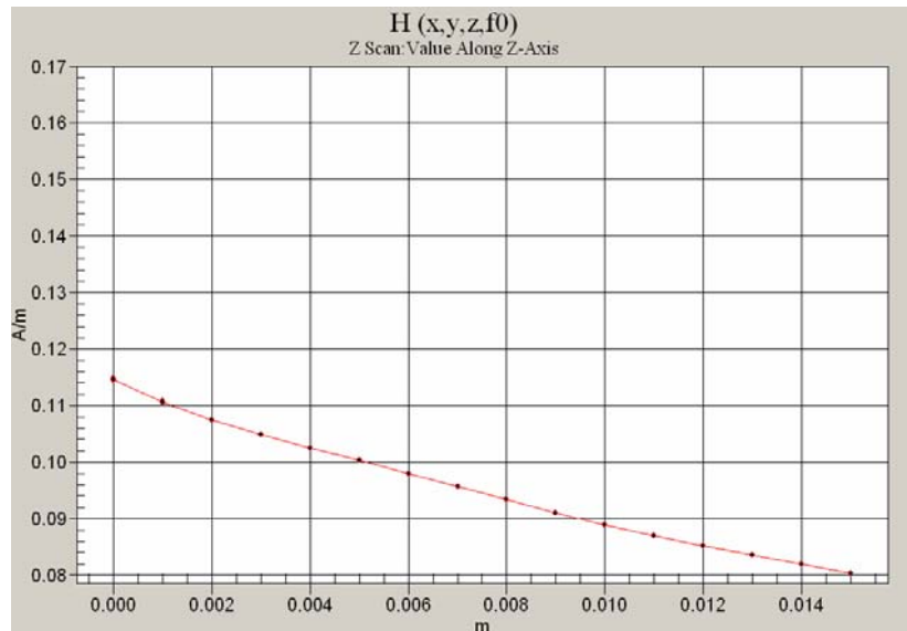
Figure 7 Z-Axis Scan at maximum point above a wireless device for H-field
