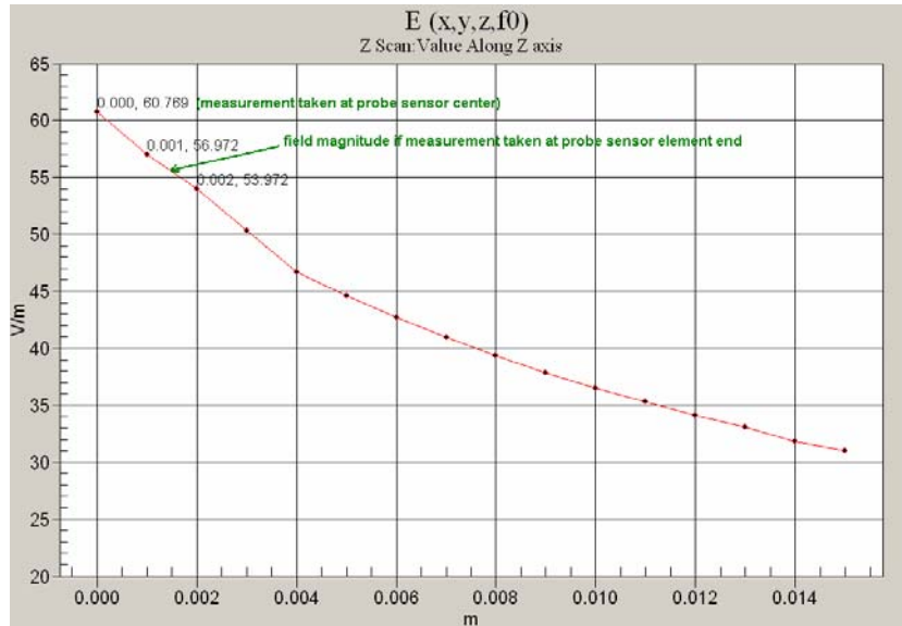
Figure 6 Z-axis scan at maximum point above a wireless device for E-field
