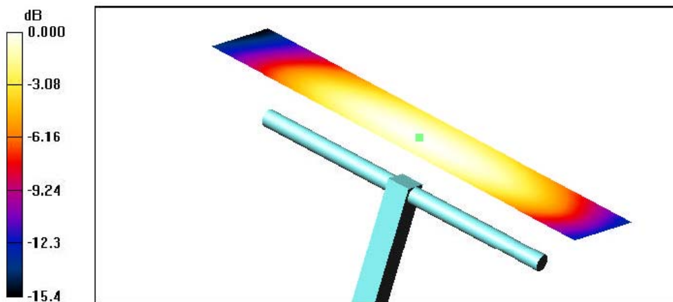
0 dB = 0.433A/m
