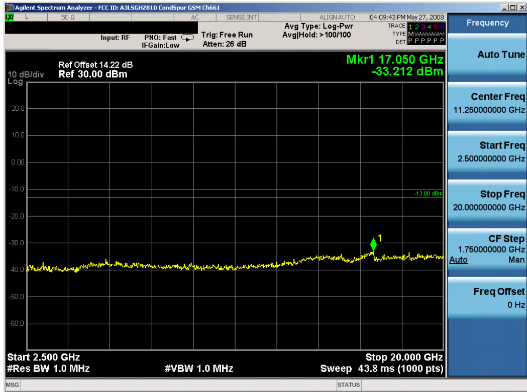
Plot 7-5. Conducted Spur Plot (PCS GSM Mode – Ch. 661)
