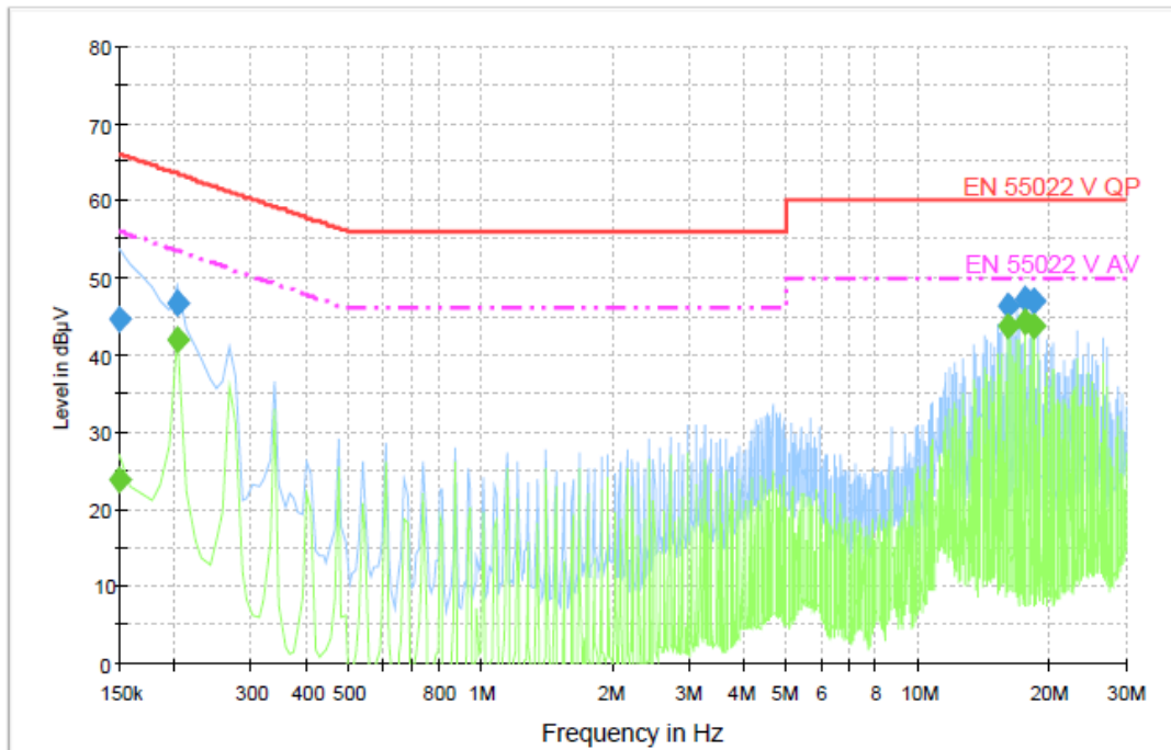
Voltage with ENV216_Class B
