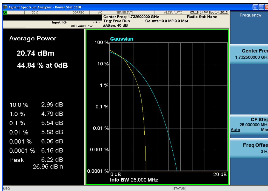
Plot 7-68. Peak to Average Ratio Plot (16QAM - RB Size 75)
