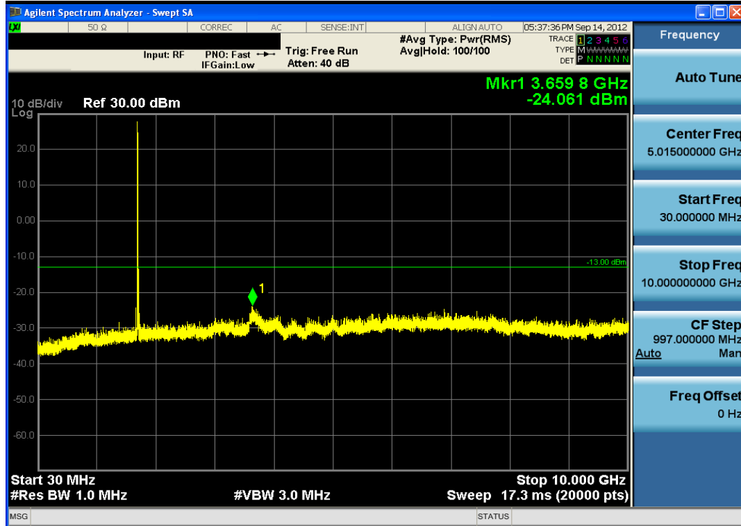
Plot 7-69. Conducted Spurious Plot (QPSK – RB Size 1, RB Offset 0– Low Channel)
