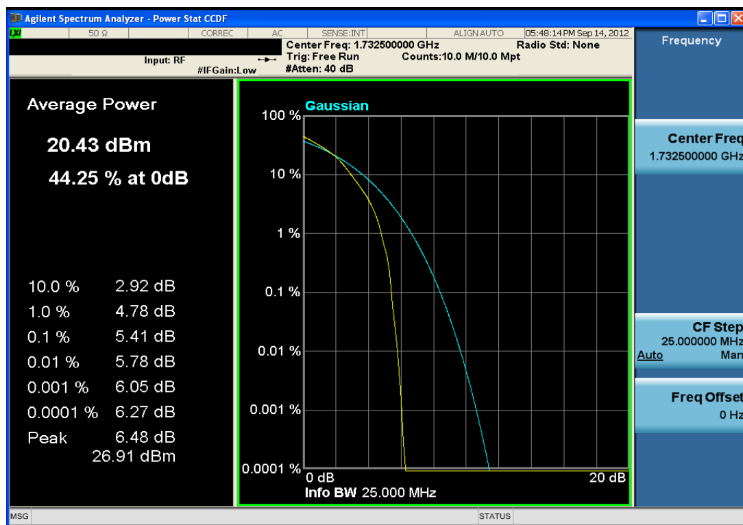
Plot 7-68. Peak to Average Ratio Plot (16QAM - RB Size 100)
