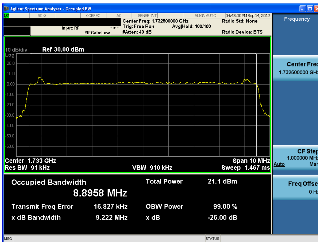
Plot 7-66. Occupied Bandwidth Plot (16-QAM – RB Size 50)
