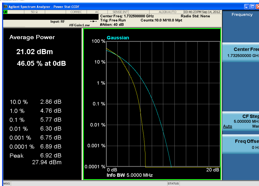
Plot 7-54. Peak to Average Ratio Plot (16QAM - RB Size 25)
