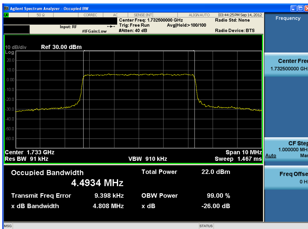
Plot 7-51. Occupied Bandwidth Plot (QPSK – RB Size 25)
