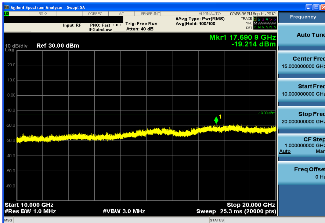
Plot 7-58. Conducted Spurious Plot (QPSK – RB Size 1, RB Offset 0 – Mid Channel)
