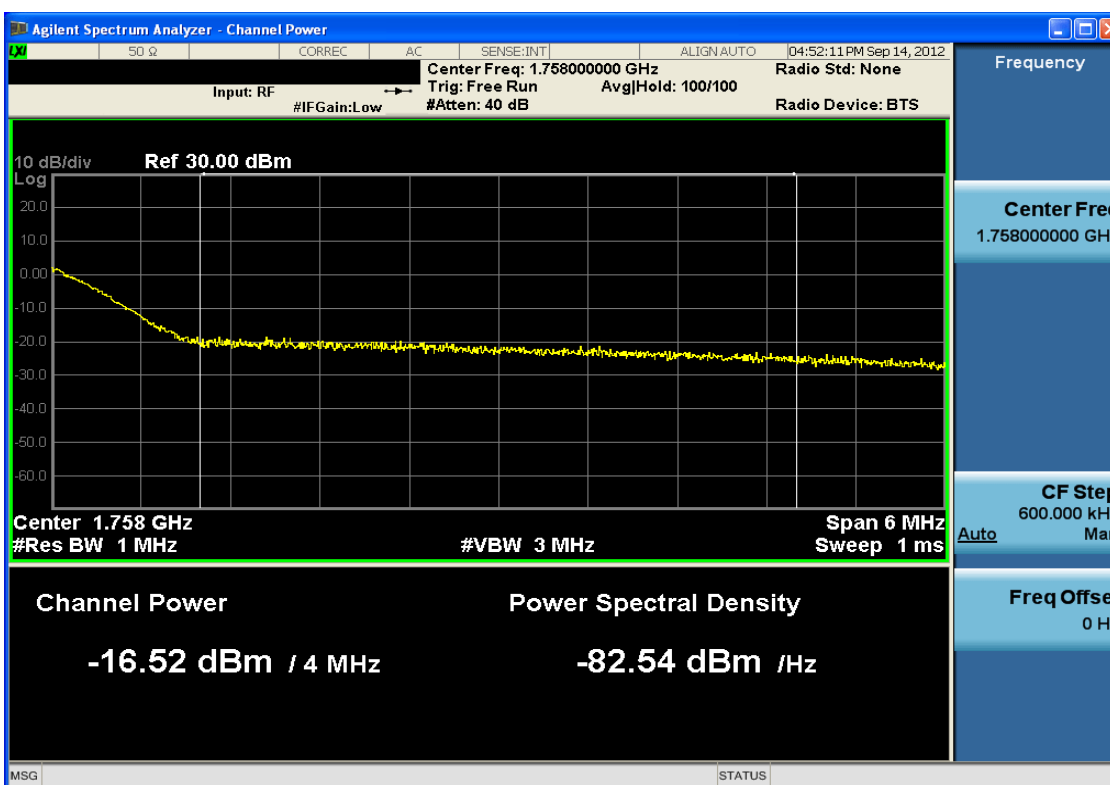
Plot 7-76. Upper Band Edge Plot (QPSK – RB Size 50)
