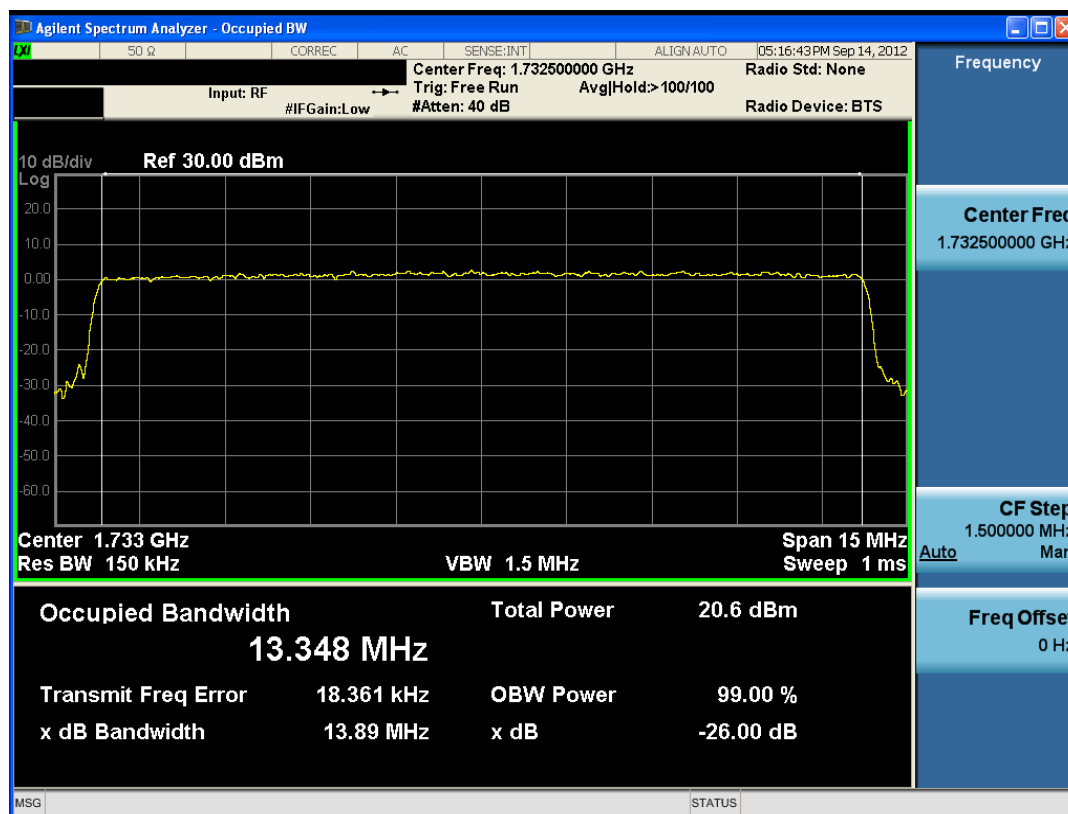
Plot 7-66. Occupied Bandwidth Plot (16-QAM – RB Size 75)
