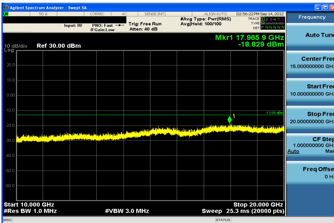
Plot 7-60. Conducted Spurious Plot (QPSK – RB Size 1, RB Offset 0 – High Channel)
