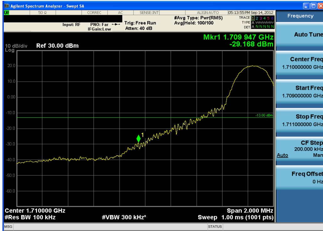
Plot 7-63. Lower Band Edge Plot (QPSK – RB Size 1, Offset 0)
