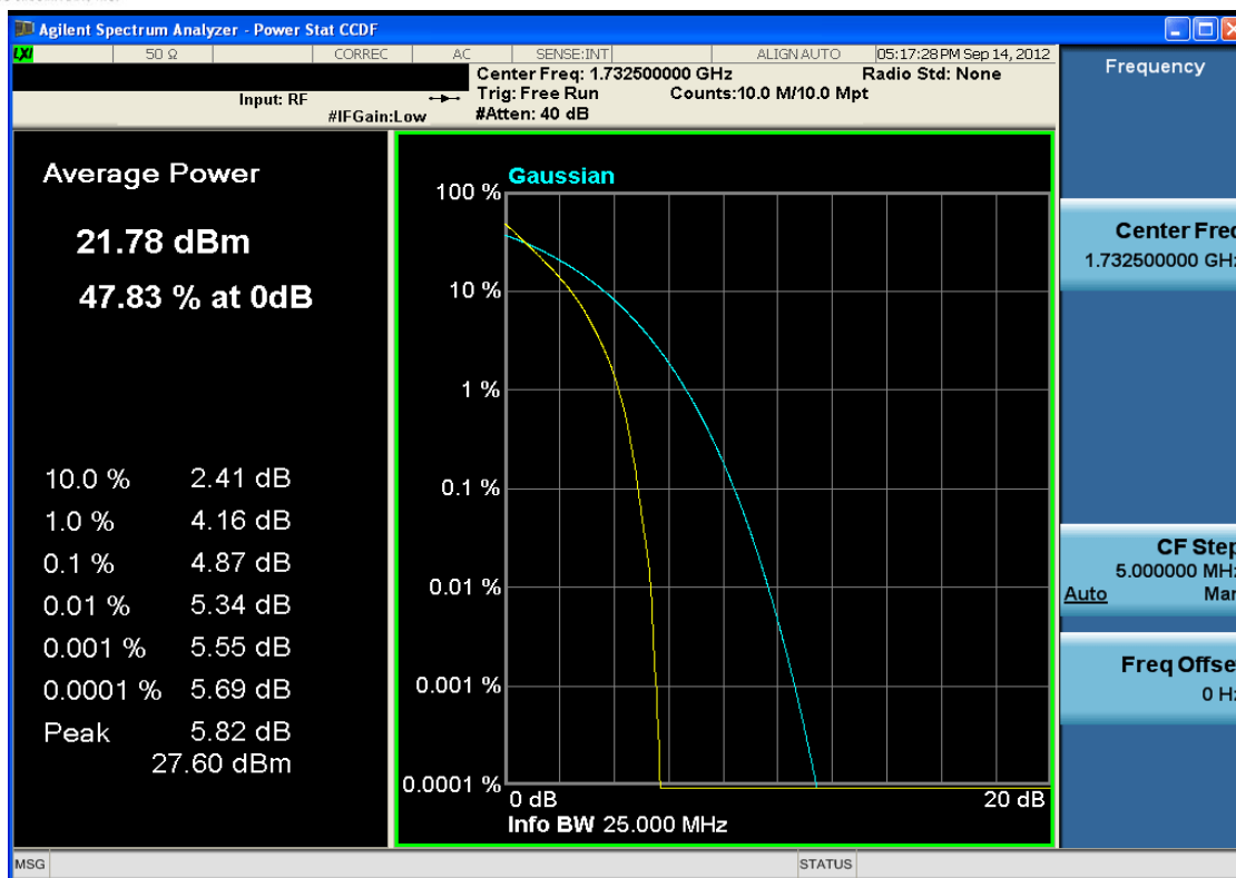
Plot 7-67. Peak to Average Ratio Plot (QPSK - RB Size 75)
