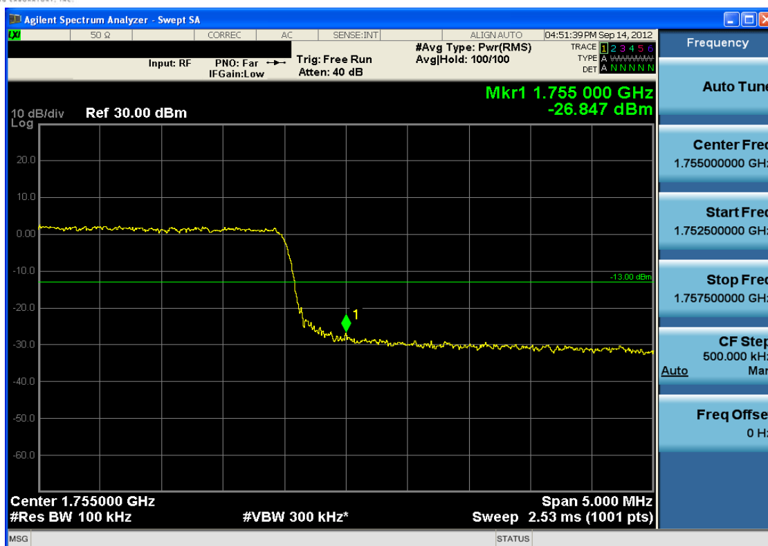
Plot 7-75. Upper Band Edge Plot (QPSK – RB Size 50)
