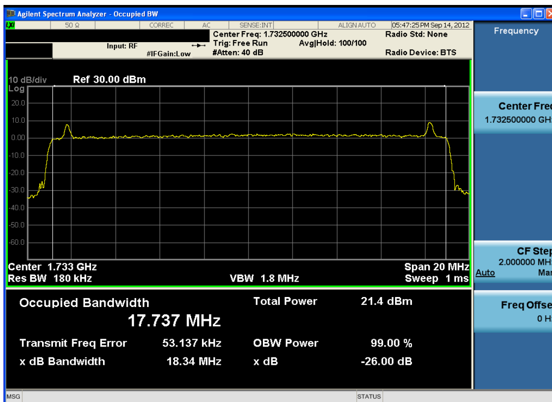
Plot 7-66. Occupied Bandwidth Plot (16-QAM – RB Size 100)
