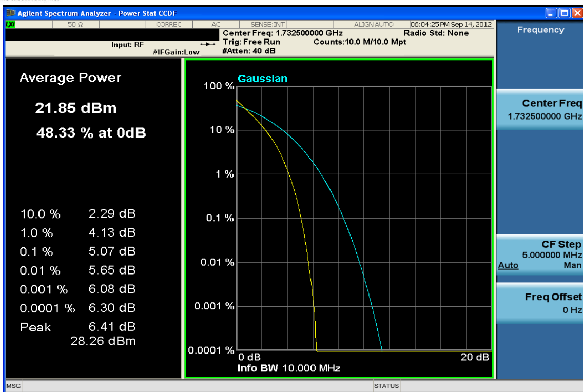
Plot 7-67. Peak to Average Ratio Plot (QPSK - RB Size 50)
