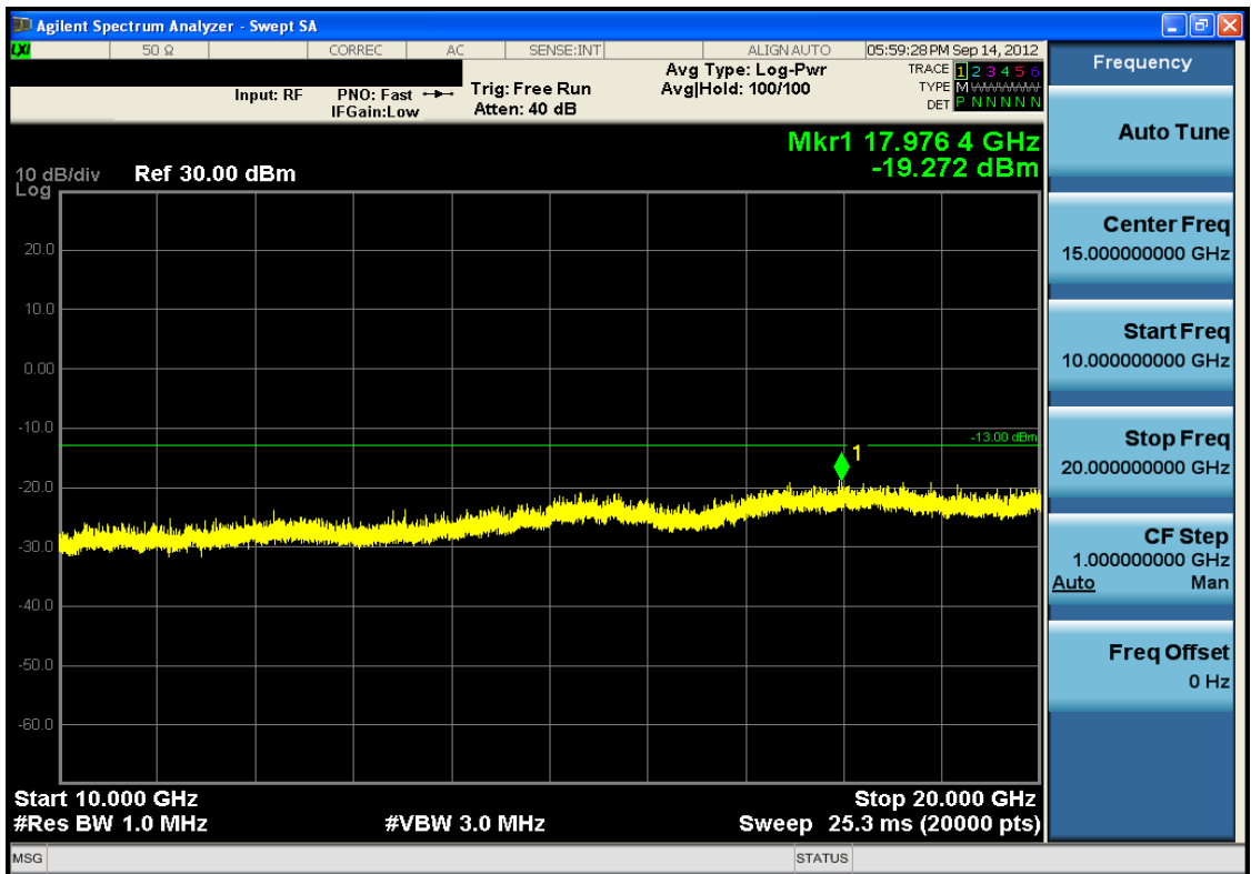
Plot 7-70. Conducted Spurious Plot (QPSK – RB Size 1, RB Offset 0 – Low Channel)
