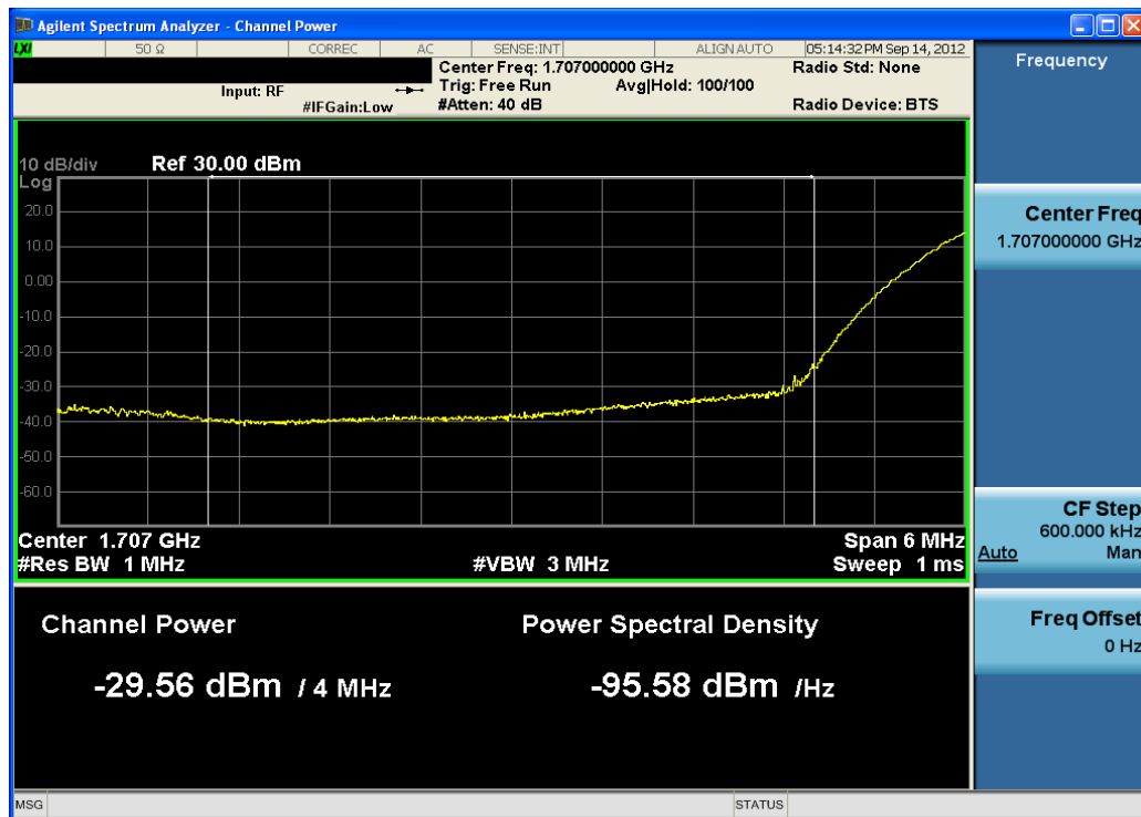
Plot 7-64. Lower Band Edge Plot (QPSK – RB Size 1, Offset 0)
