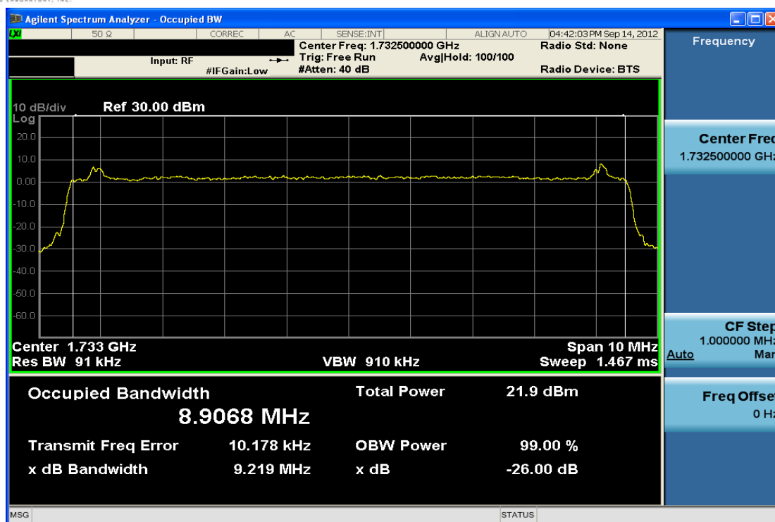
Plot 7-65. Occupied Bandwidth Plot (QPSK – RB Size 50)
