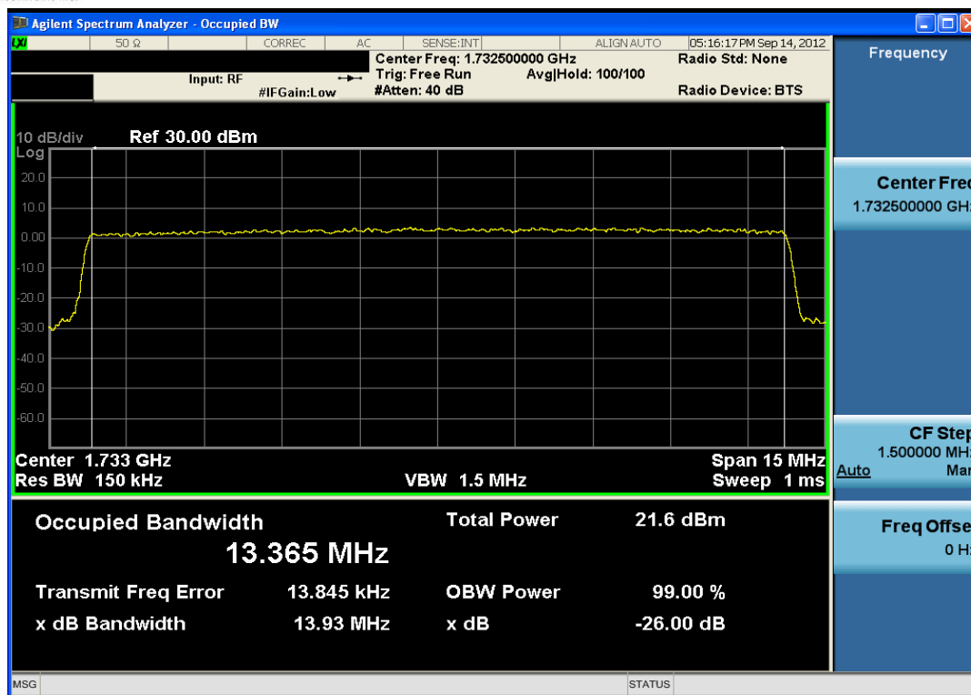
Plot 7-65. Occupied Bandwidth Plot (QPSK – RB Size 75)
