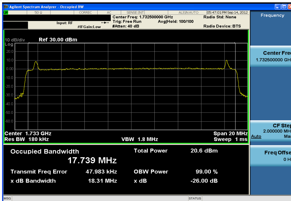
Plot 7-65. Occupied Bandwidth Plot (QPSK – RB Size 100)
