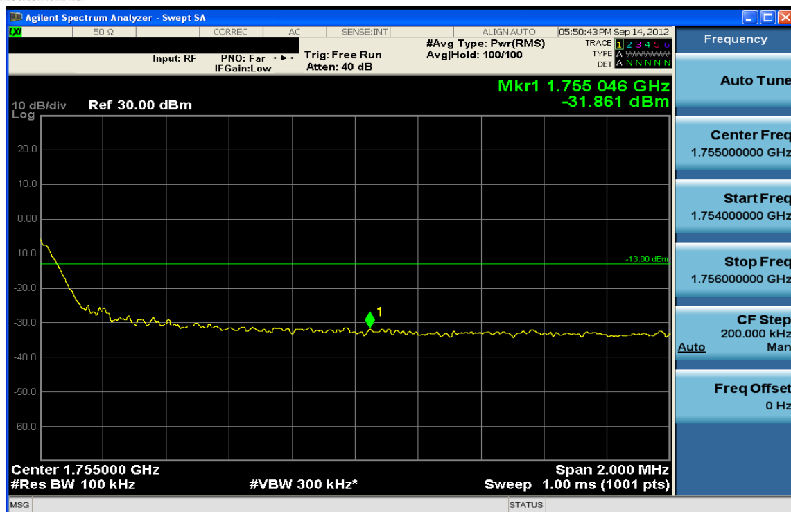
Plot 7-75. Upper Band Edge Plot (QPSK – RB Size 1, Offset 99)
