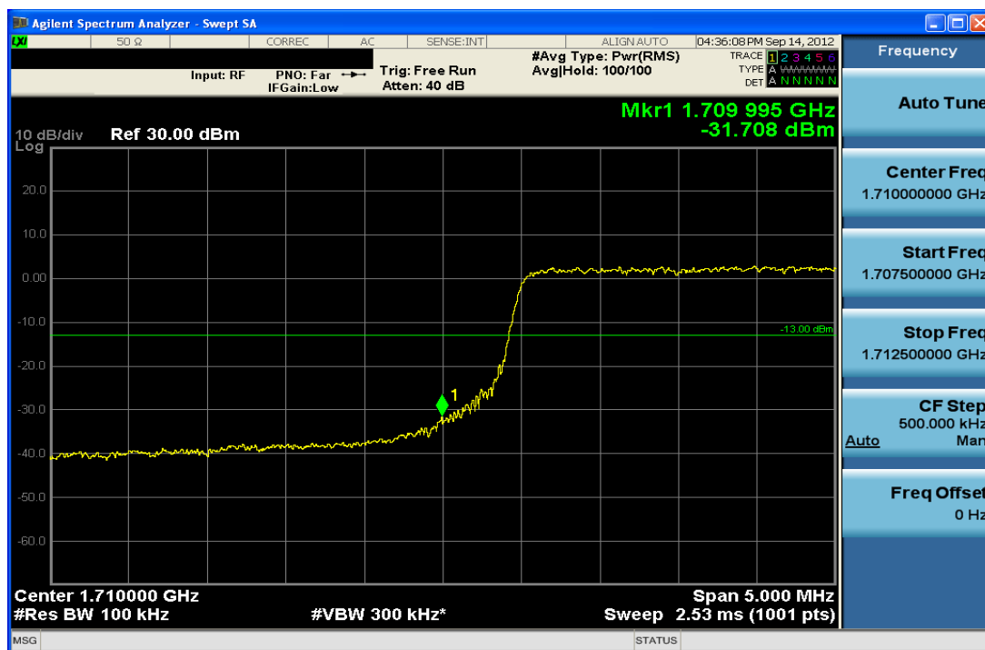
Plot 7-63. Lower Band Edge Plot (QPSK – RB Size 50)
