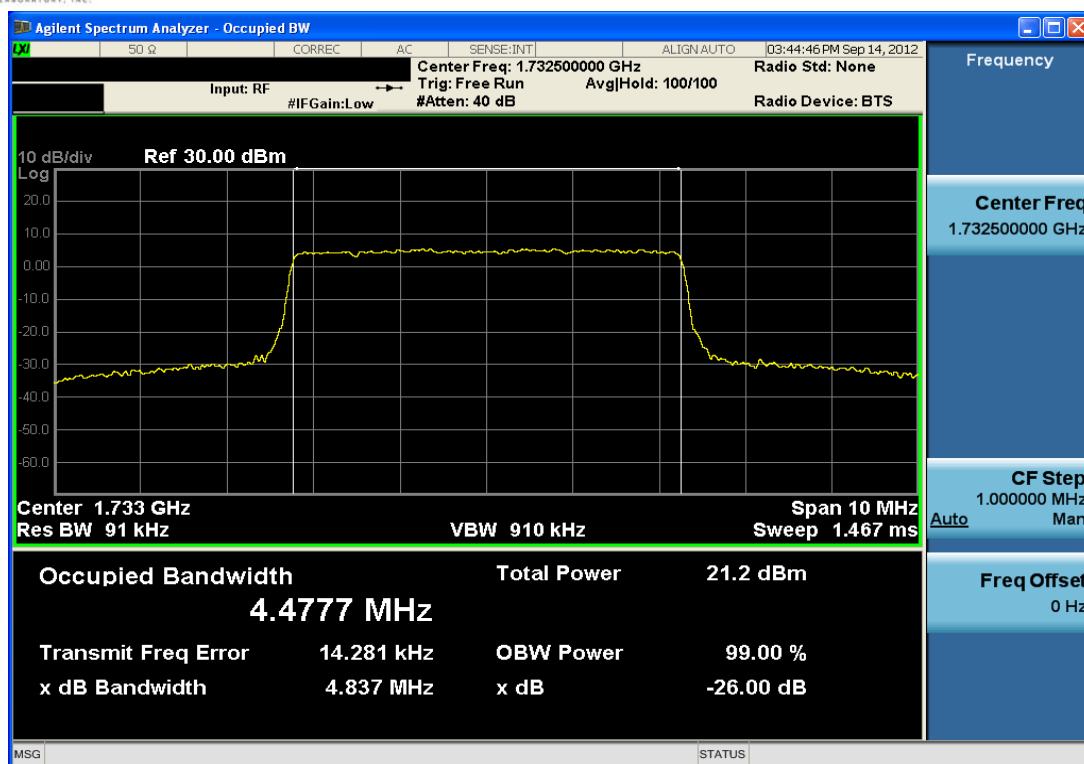
Plot 7-52. Occupied Bandwidth Plot (16-QAM – RB Size 25)
