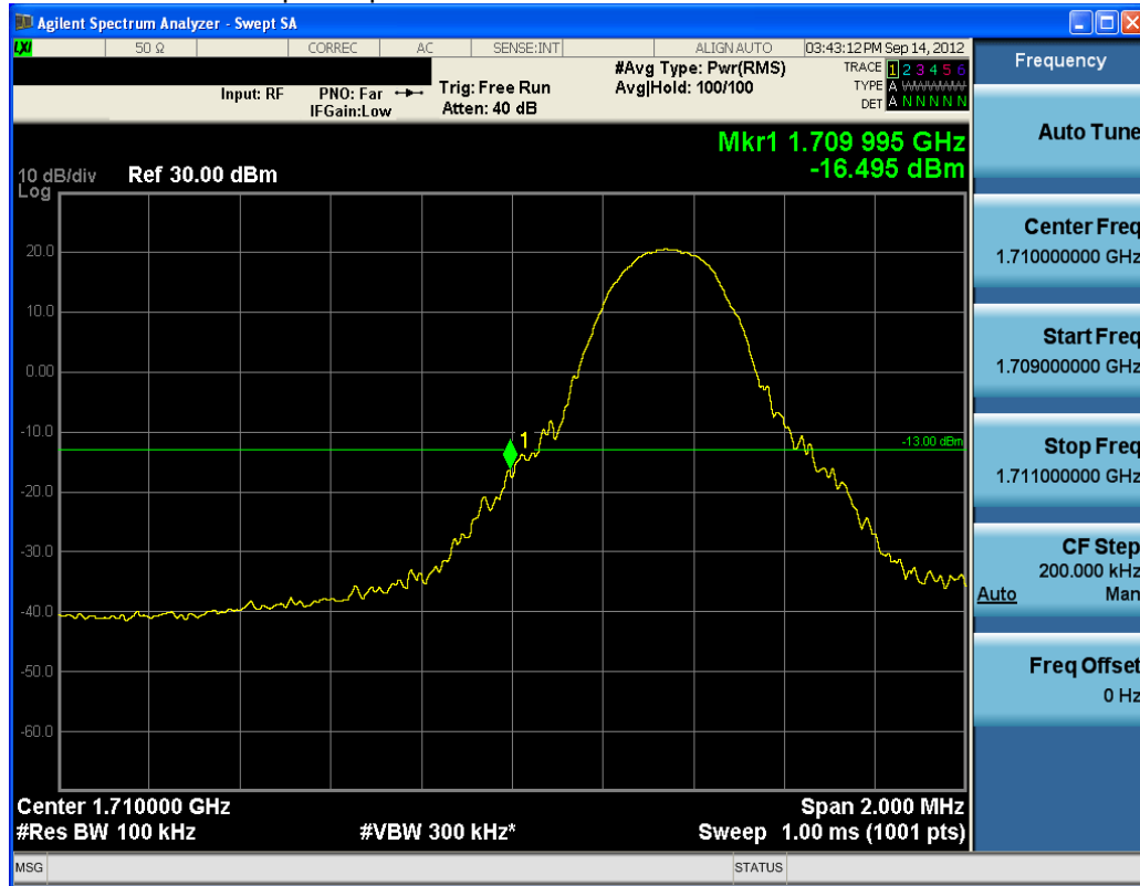
Plot 7-49. Lower Band Edge Plot (QPSK – RB Size 25)
