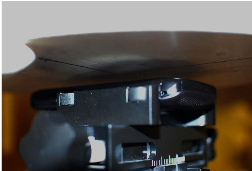
Figure 21-6 SAR Test Setup Photo – Front at 1.0 cm
