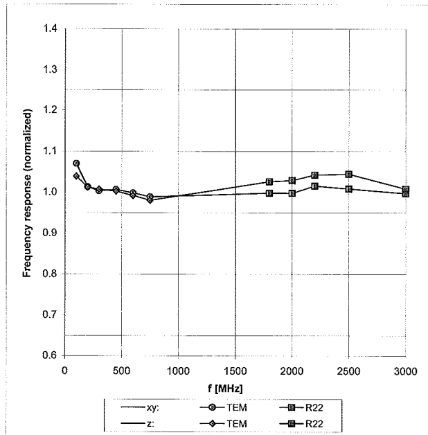
Uncertainty of Frequency Response of H-field: ± 6.3% (k=2)
