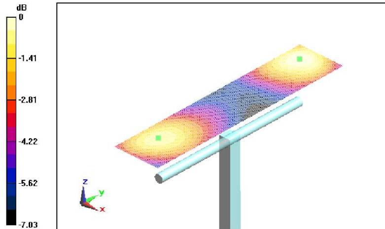
0 dB = 145.1V/m
