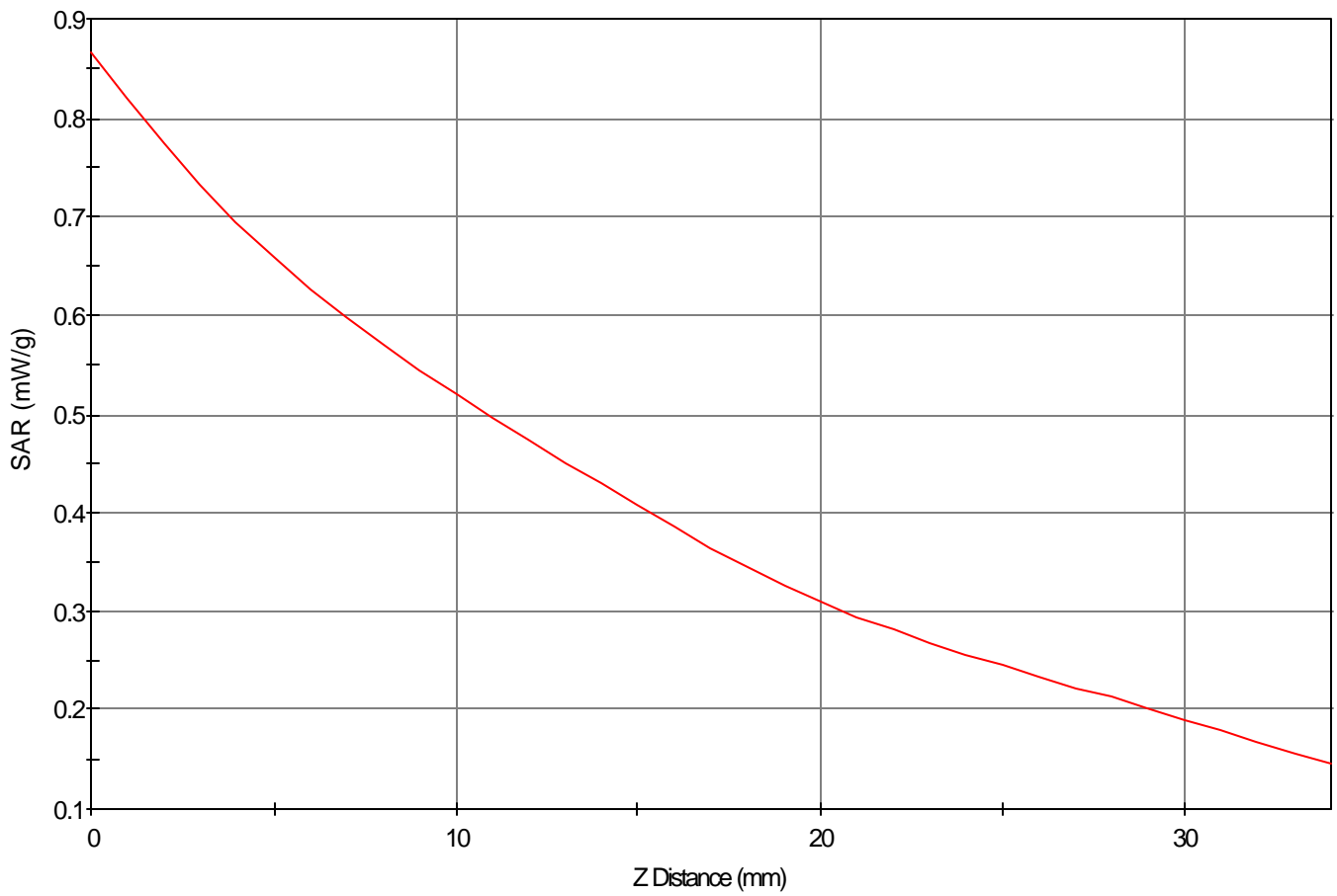
SAR - Z Axis at Hotspot x:60.0 y:14.0
