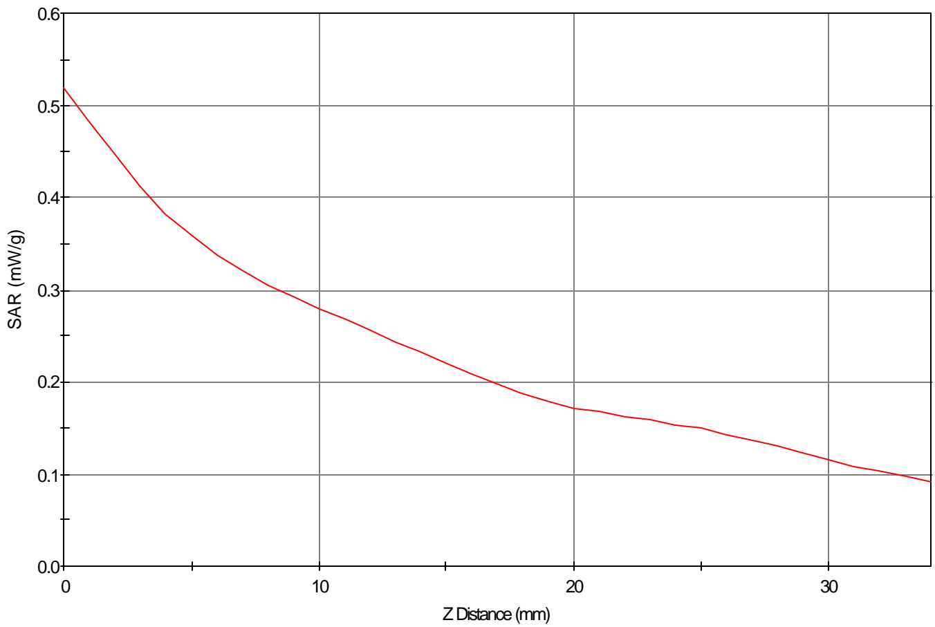
SAR - Z Axis at Hotspot x:60.0 y:16.0
