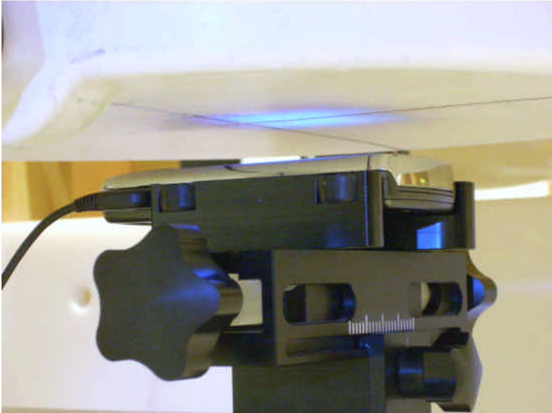
Figure 13: Body SAR, Front Side with 15mm Space
