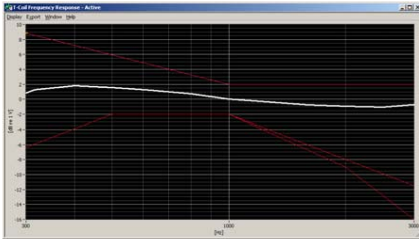
Figure 7-1 Axial Frequency Response
