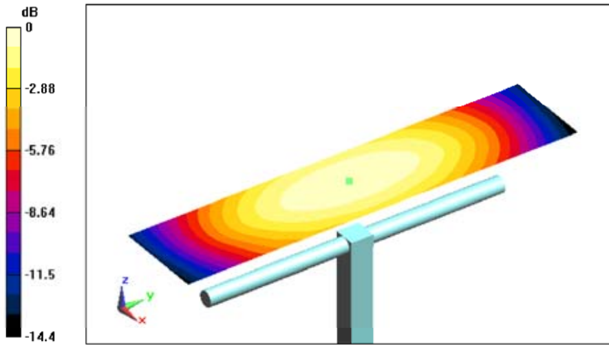
0 dB = 0.419A/m
