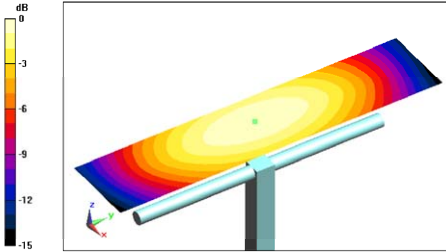
0 dB = 0.449A/m
