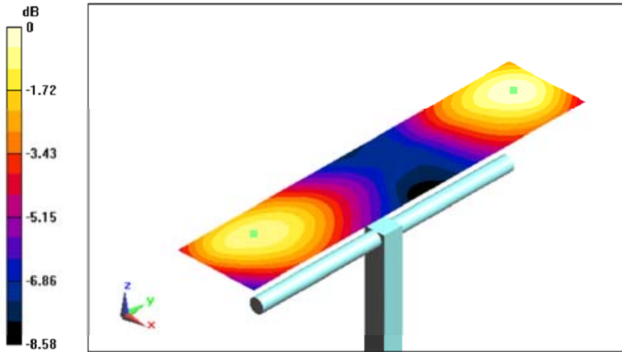
0 dB = 143.8V/m
